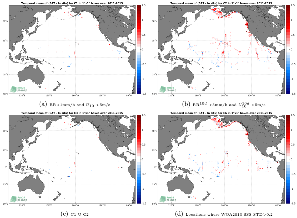
Figure 12: Temporal mean gridded over spatial boxes of size 1^\circ \times 1^\circ of \Delta SSS (Aquarius-L3-JPL-V5-7DAY-RUNNING - TSG-SAMOS) for 4 different subdatasets corresponding to: RR > 1mm/h and U_{10} < 5\text{m/s} (a), RR^{10d} > 5\text{mm/h} and U_{10}^{10d} < 5\text{m/s} (b), C1 U C2 (c), Locations where WOA2013 SSS STD > 0.2 (d).
