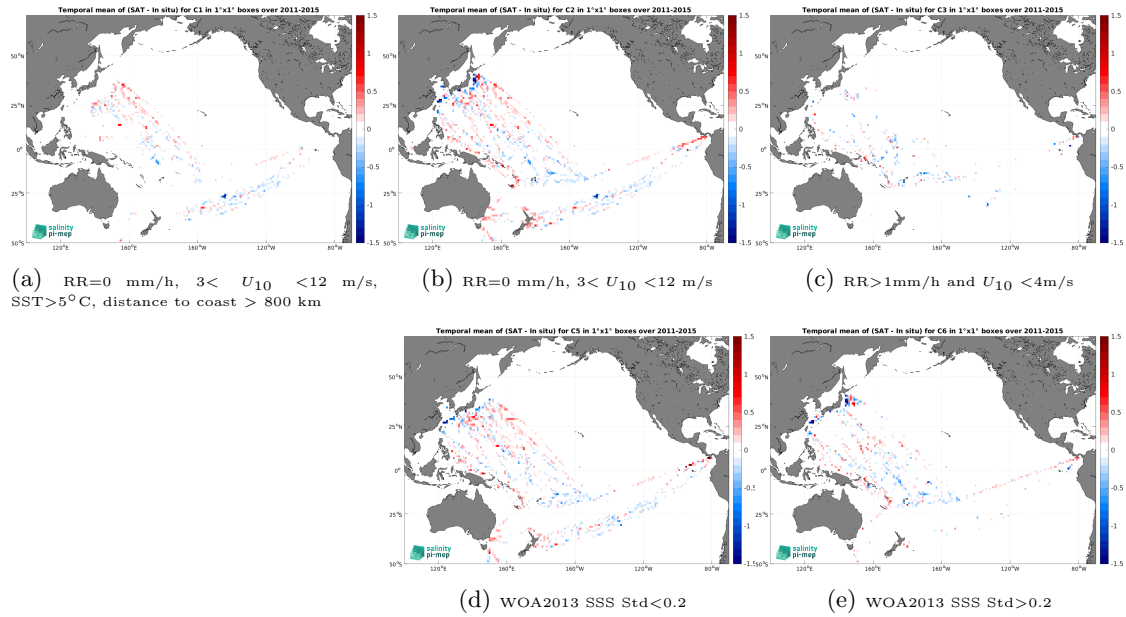
Figure 12: Temporal mean gridded over spatial boxes of size 1^\circ \times 1^\circ of \Delta\text{SSS} (Aquarius SSS L3 CAP v5 - 7-Day running (JPL) - TSG (LEGOS-DM)) for 5 different subdatasets corresponding to:RR=0 mm/h, 3 < U_{10} < 12 m/s, SST >5^\circ\text{C} , distance to coast > 800 km (a), RR=0 mm/h, 3 < U_{10} < 12 m/s (b), RR >1 mm/h and U_{10} < 4 m/s (c), WOA2013 SSS Std <0.2 (d), WOA2013 SSS Std >0.2 (e).
