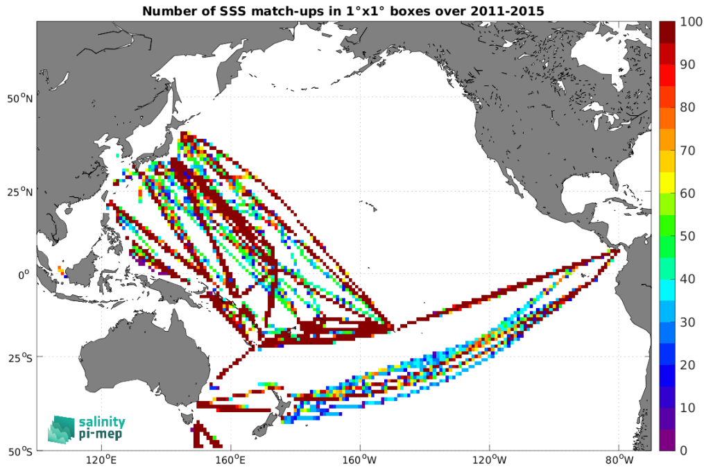
Figure 4: Number of SSS match-ups between TSG (LEGOS-DM) SSS and the Aquarius SSS L3 CAP v5 - 7-Day running (JPL) SSS product for the Pacific Ocean Pi-MEP region over 1^\circ \times 1^\circ boxes and for the full satellite product period.
