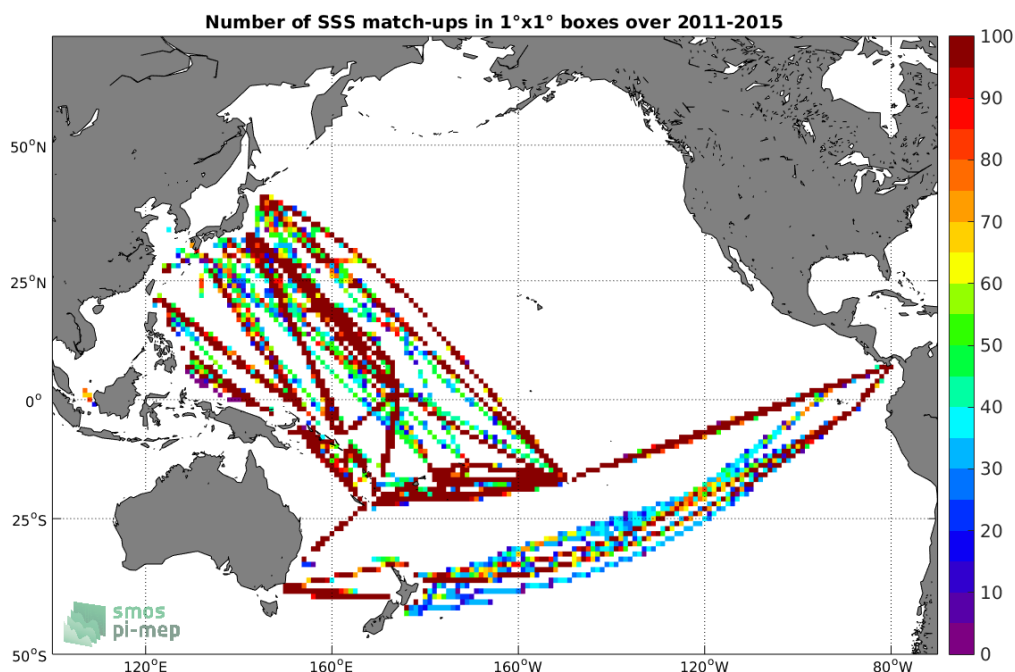
Figure 4: Number of SSS match-ups between TSG-LEGOS-DM SSS and the Aquarius-L3-JPL-V5-7DAY-RUNNING SSS product for the Pacific Ocean Pi-MEP region over 1^\circ \times 1^\circ boxes and for the full satellite product period.
