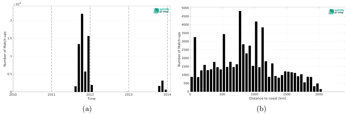
Figure 2: Number of match-ups between TSG (GOSUD-Sailing-ship) and Aquarius SSS L3 CAP v5 - 7-Day running (JPL) SSS as a function of time (a) and as function of the distance to coast (b) over the Pacific Ocean Pi-MEP region and for the full satellite product period.
