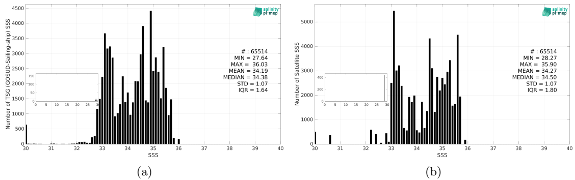
Figure 3: Histograms of SSS from TSG (GOSUD-Sailing-ship) (a) and Aquarius SSS L3 CAP v5 - 7-Day running (JPL) (b) considering all match-up pairs per bins of 0.1 over the Pacific Ocean Pi-MEP region and for the full satellite product period.
