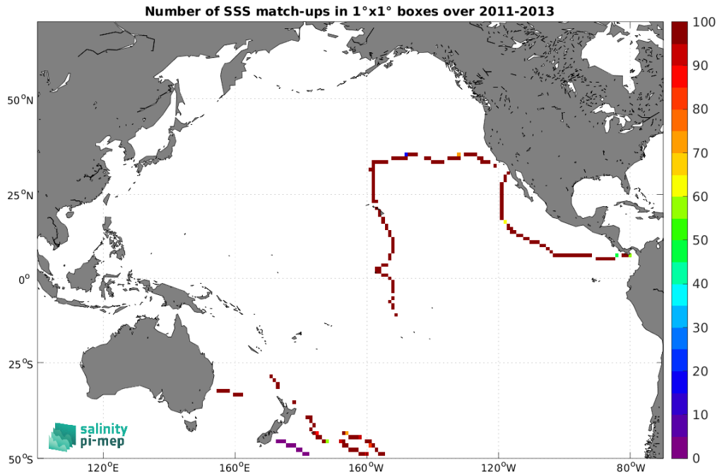
Figure 5: Number of SSS match-ups between TSG (GOSUD-Sailing-ship) SSS and the Aquarius SSS L3 CAP v5 - 7-Day running (JPL) SSS product for the Pacific Ocean Pi-MEP region over 1^\circ \times 1^\circ boxes and for the full satellite product period.
