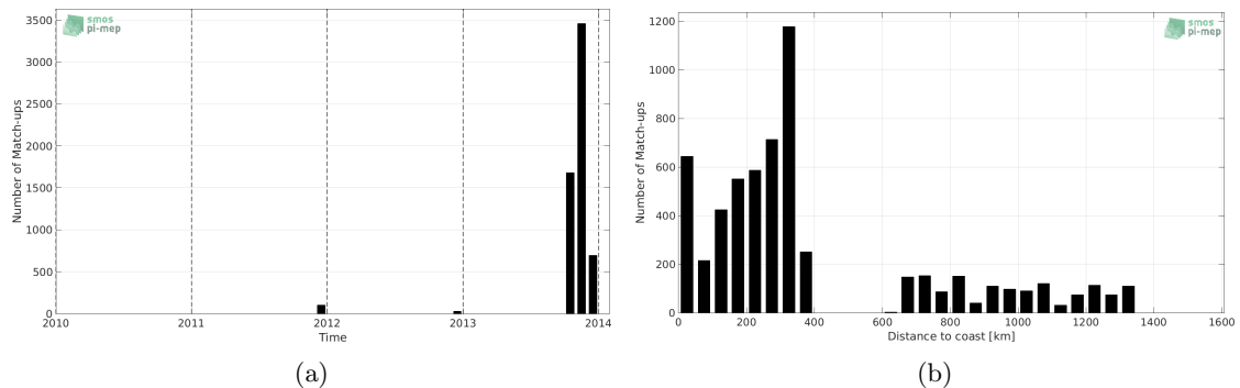
Figure 1: Number of match-ups between TSG-GOSUD-Sailing-ship and Aquarius-L3-JPL-V5-7DAY-RUNNING SSS as a function of time (a) and as function of the distance to coast (b) over the Pacific Ocean Pi-MEP region and for the full satellite product period.
