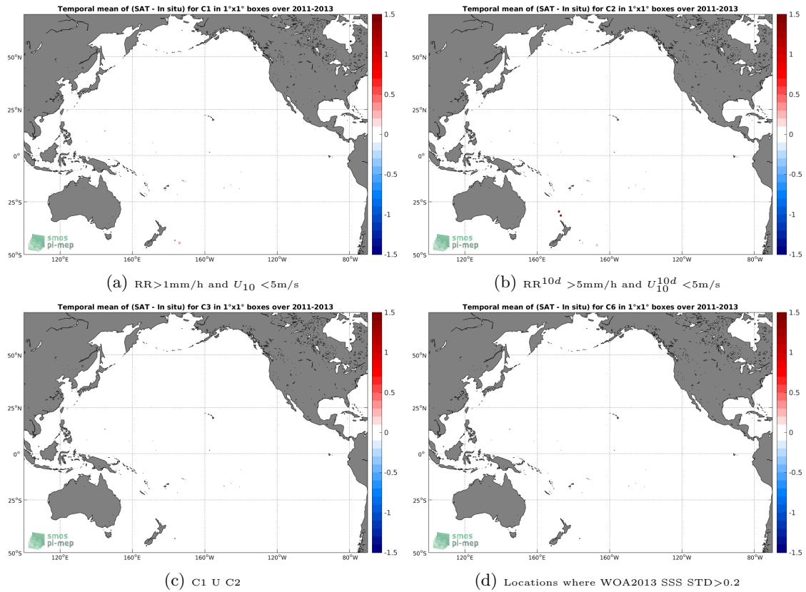
Figure 12: Temporal mean gridded over spatial boxes of size 1^\circ \times 1^\circ of \Delta SSS (Aquarius-L3-JPL-V5-7DAY-RUNNING - TSG-GOSUD-Sailing-ship) for 4 different subdatasets corresponding to: RR > 1\text{mm/h} and U_{10} < 5\text{m/s} (a), RR^{10d} > 5\text{mm/h} and U_{10}^{10d} < 5\text{m/s} (b), C1 U C2 (c), Locations where WOA2013 SSS STD > 0.2 (d).
