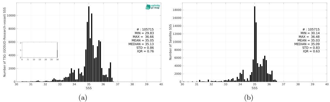
Figure 3: Histograms of SSS from TSG (GOSUD-Research-vessel) (a) and Aquarius SSS L3 CAP v5 - 7-Day running (JPL) (b) considering all match-up pairs per bins of 0.1 over the Pacific Ocean Pi-MEP region and for the full satellite product period.
