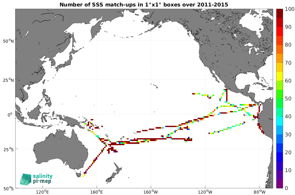
Figure 5: Number of SSS match-ups between TSG (GOSUD-Research-vessel) SSS and the Aquarius SSS L3 CAP v5 - 7-Day running (JPL) SSS product for the Pacific Ocean Pi-MEP region over 1^\circ \times 1^\circ boxes and for the full satellite product period.
