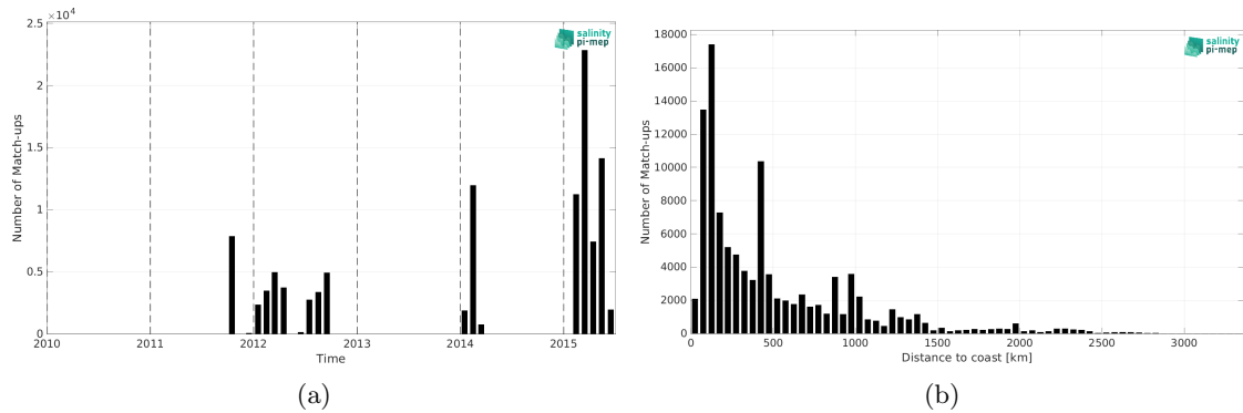
Figure 2: Number of match-ups between TSG (GOSUD-Research-vessel) and Aquarius SSS L3 CAP v5 - 7-Day running (JPL) SSS as a function of time (a) and as function of the distance to coast (b) over the Pacific Ocean Pi-MEP region and for the full satellite product period.
