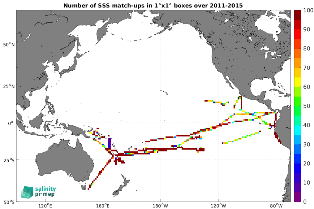
Figure 4: Number of SSS match-ups between TSG (GOSUD-Research-vessel) SSS and the Aquarius SSS L3 CAP v5 - 7-Day running (JPL) SSS product for the Pacific Ocean Pi-MEP region over 1^\circ \times 1^\circ boxes and for the full satellite product period.
