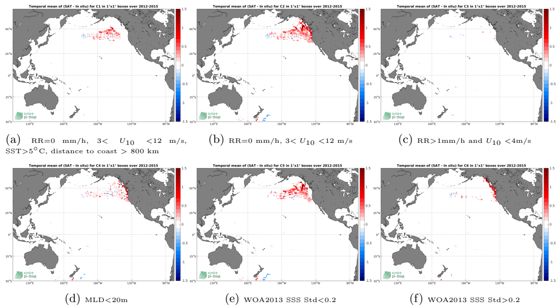
Figure 12: Temporal mean gridded over spatial boxes of size 1^\circ \times 1^\circ of \Delta SSS (Aquarius-L3-JPL-V5-7DAY-RUNNING - Sea mammals) for 6 different subdatasets corresponding to:RR=0 mm/h, 3 < U_{10} < 12 m/s, SST >5^\circ C, distance to coast > 800 km (a), RR=0 mm/h, 3 < U_{10} < 12 m/s (b), RR >1 mm/h and U_{10} < 4 m/s (c),MLD <20 m (d),WOA2013 SSS Std <0.2 (e),WOA2013 SSS Std >0.2 (f).
