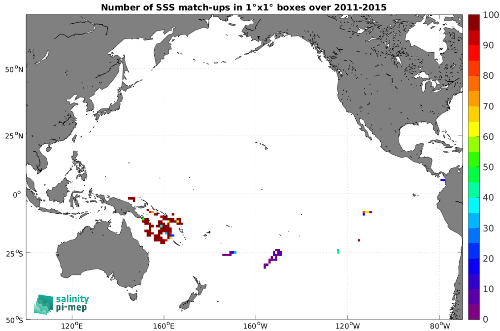
Figure 4: Number of SSS match-ups between Surface drifters SSS and the Aquarius SSS L3 CAP v5 - 7-Day running (JPL) SSS product for the Pacific Ocean Pi-MEP region over 1^\circ \times 1^\circ boxes and for the full satellite product period.
