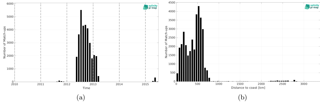
Figure 2: Number of match-ups between Surface drifters and Aquarius SSS L3 CAP v5 - 7-Day running (JPL) SSS as a function of time (a) and as function of the distance to coast (b) over the Pacific Ocean Pi-MEP region and for the full satellite product period.
