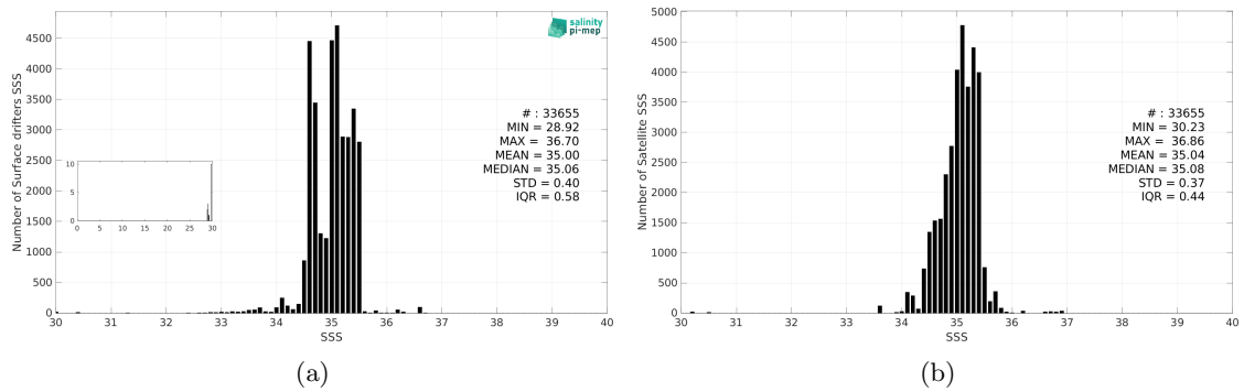
Figure 3: Histograms of SSS from Surface drifters (a) and Aquarius SSS L3 CAP v5 - 7-Day running (JPL) (b) considering all match-up pairs per bins of 0.1 over the Pacific Ocean Pi-MEP region and for the full satellite product period.
