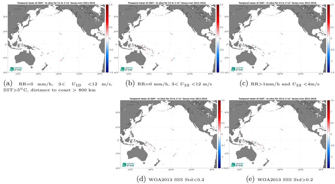
Figure 13: Temporal mean gridded over spatial boxes of size 1^\circ \times 1^\circ of \Delta SSS (Aquarius SSS L3 CAP v5 - 7-Day running (JPL) - Surface drifters) for 5 different subdatasets corresponding to:RR=0 mm/h, 3 < U_{10} < 12 m/s, SST >5^\circ\text{C} , distance to coast > 800 km (a), RR=0 mm/h, 3 < U_{10} < 12 m/s (b), RR >1 mm/h and U_{10} < 4 m/s (c), WOA2013 SSS Std <0.2 (d), WOA2013 SSS Std >0.2 (e).
