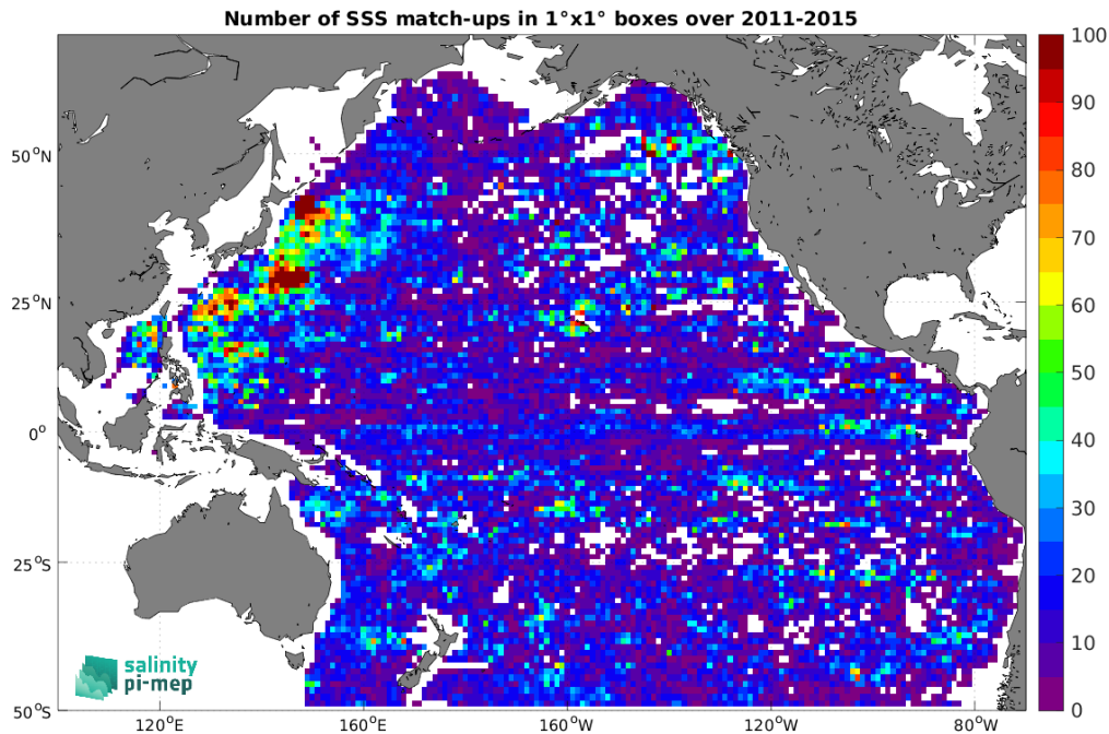
Figure 4: Number of SSS match-ups between Argo SSS and the Aquarius SSS L3 CAP v5 - 7-Day running (JPL) SSS product for the Pacific Ocean Pi-MEP region over 1^\circ \times 1^\circ boxes and for the full satellite product period.
