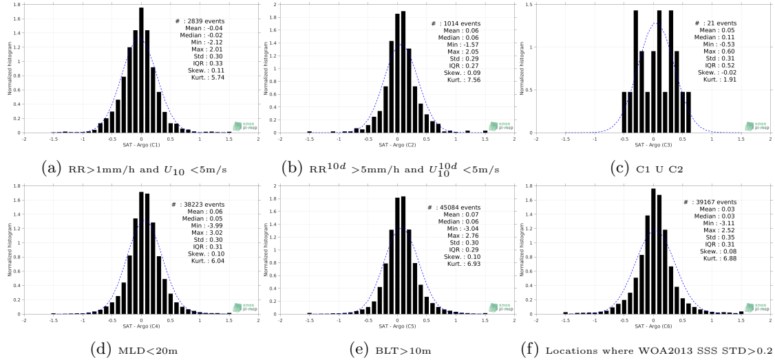
Figure 13: Normalized histogram of \Delta SSS (Aquarius-L3-JPL-V5-7DAY-RUNNING - Argo) for 6 different subdatasets corresponding to: RR>1mm/h and U_{10} <5m/s (a), RR 10d >5mm/h and U_{10}^{10d} <5m/s (b), C1 U C2 (c),MLD<20m (d),BLT>10m (e),Locations where WOA2013 SSS STD>0.2 (f).
