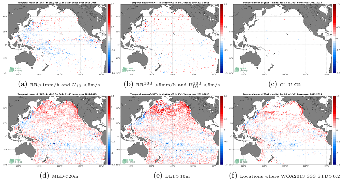
Figure 12: Temporal mean gridded over spatial boxes of size 1^\circ \times 1^\circ of \Delta\text{SSS} (Aquarius-L3-JPL-V5-7DAY-RUNNING - Argo) for 6 different subdatasets corresponding to: RR > 1\text{mm/h} and U_{10} < 5\text{m/s} (a), RR^{10d} > 5\text{mm/h} and U_{10}^{10d} < 5\text{m/s} (b), C1 U C2 (c), MLD < 20\text{m} (d), BLT > 10\text{m} (e), Locations where WOA2013 SSS STD > 0.2 (f).
