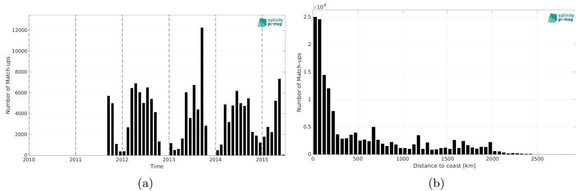
Figure 2: Number of match-ups between TSG (SAMOS) and Aquarius SSS L3 CAP v5 - Monthly (JPL) SSS as a function of time (a) and as function of the distance to coast (b) over the Pacific Ocean Pi-MEP region and for the full satellite product period.
