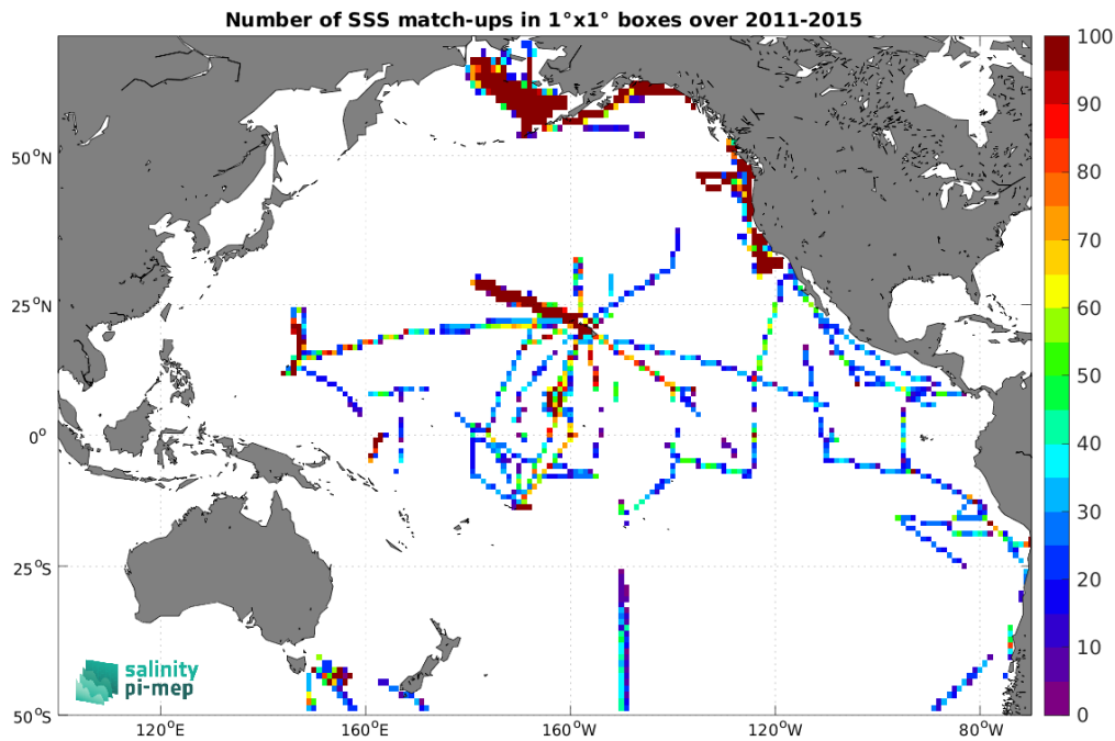
Figure 5: Number of SSS match-ups between TSG (SAMOS) SSS and the Aquarius SSS L3 CAP v5 - Monthly (JPL) SSS product for the Pacific Ocean Pi-MEP region over 1^\circ \times 1^\circ boxes and for the full satellite product period.
