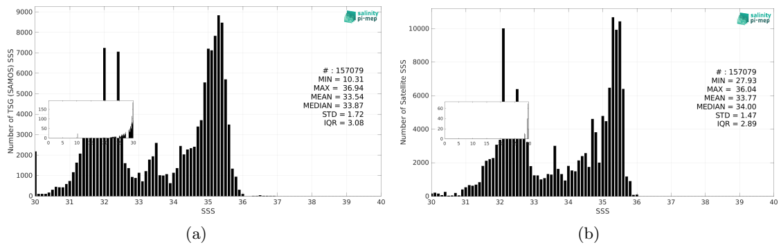
Figure 3: Histograms of SSS from TSG (SAMOS) (a) and Aquarius SSS L3 CAP v5 - Monthly (JPL) (b) considering all match-up pairs per bins of 0.1 over the Pacific Ocean Pi-MEP region and for the full satellite product period.
