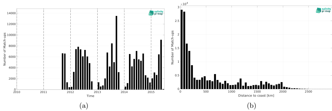
Figure 1: Number of match-ups between TSG (SAMOS) and Aquarius SSS L3 CAP v5 - Monthly (JPL) SSS as a function of time (a) and as function of the distance to coast (b) over the Pacific Ocean Pi-MEP region and for the full satellite product period.
