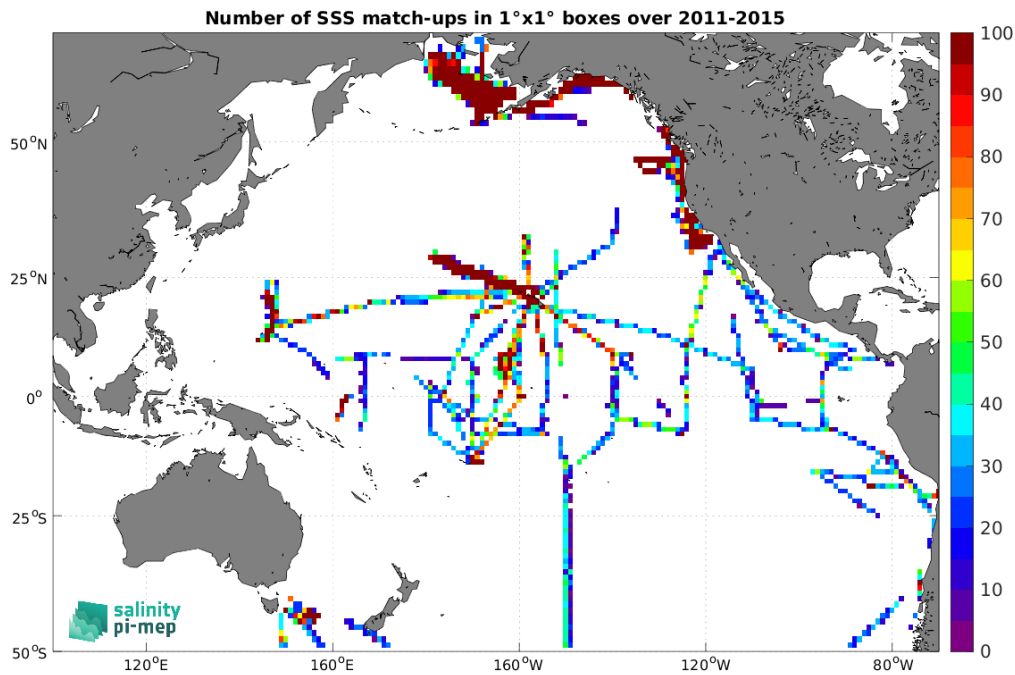
Figure 4: Number of SSS match-ups between TSG (SAMOS) SSS and the Aquarius SSS L3 CAP v5 - Monthly (JPL) SSS product for the Pacific Ocean Pi-MEP region over 1^\circ \times 1^\circ boxes and for the full satellite product period.
