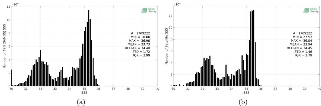
Figure 2: Histograms of SSS from TSG (SAMOS) (a) and Aquarius SSS L3 CAP v5 - Monthly (JPL) (b) considering all match-up pairs per bins of 0.1 over the Pacific Ocean Pi-MEP region and for the full satellite product period.
