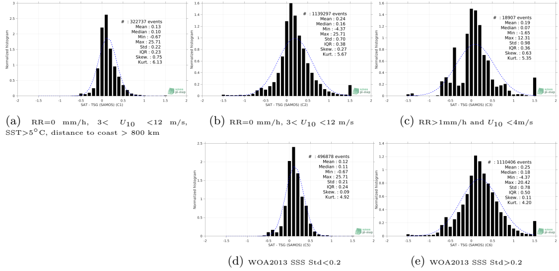
Figure 13: Normalized histogram of \Delta\text{SSS} (Aquarius SSS L3 CAP v5 - Monthly (JPL) - TSG (SAMOS)) for 5 different subdatasets corresponding to: \text{RR}=0 \text{ mm/h} , 3 < U_{10} < 12 \text{ m/s} , \text{SST} > 5^\circ\text{C} , distance to coast > 800 \text{ km} (a), \text{RR}=0 \text{ mm/h} , 3 < U_{10} < 12 \text{ m/s} (b), \text{RR} > 1 \text{ mm/h} and U_{10} < 4 \text{ m/s} (c), WOA2013 SSS Std < 0.2 (d), WOA2013 SSS Std > 0.2 (e).
