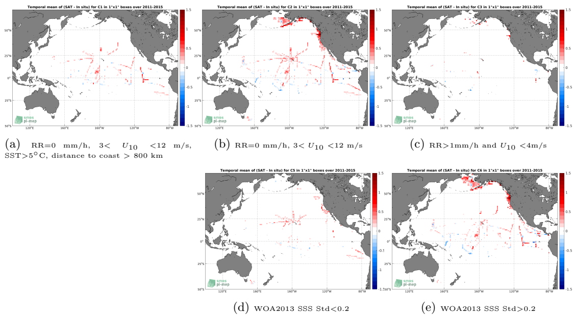
Figure 12: Temporal mean gridded over spatial boxes of size 1°x1° of \Delta SSS (Aquarius SSS L3 CAP v5 - Monthly (JPL) - TSG (SAMOS)) for 5 different subdatasets corresponding to:RR=0 mm/h, 3 < U_{10} < 12 m/s, SST > 5°C, distance to coast > 800 km (a), RR=0 mm/h, 3 < U_{10} < 12 m/s (b), RR > 1mm/h and U_{10} < 4 m/s (c), WOA2013 SSS Std < 0.2 (d), WOA2013 SSS Std > 0.2 (e).
