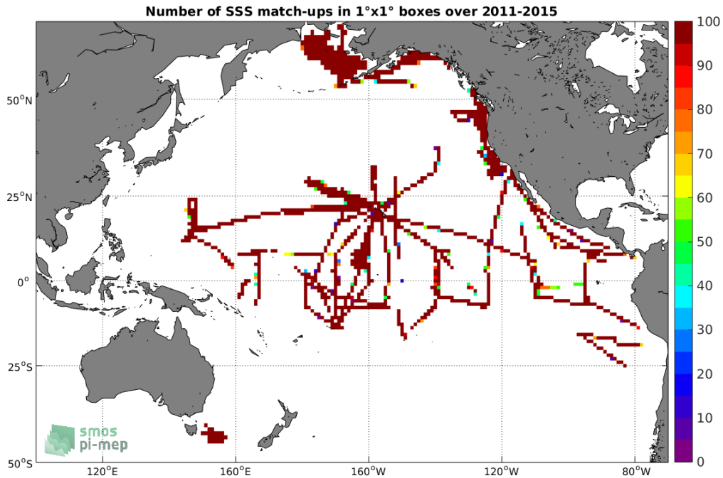
Figure 4: Number of SSS match-ups between TSG-SAMOS SSS and the Aquarius-L3-JPL-V5-MONTHLY SSS product for the Pacific Ocean Pi-MEP region over 1^\circ \times 1^\circ boxes and for the full satellite product period.
