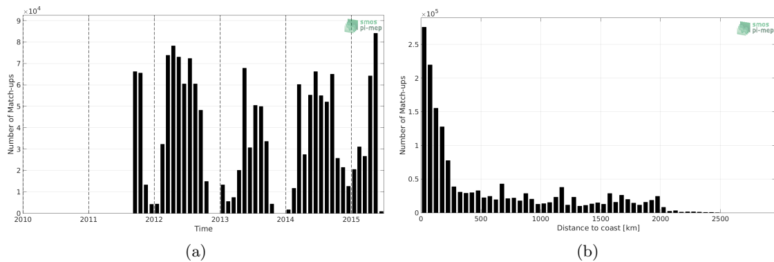
Figure 1: Number of match-ups between TSG-SAMOS and Aquarius-L3-JPL-V5-MONTHLY SSS as a function of time (a) and as function of the distance to coast (b) over the Pacific Ocean Pi-MEP region and for the full satellite product period.
