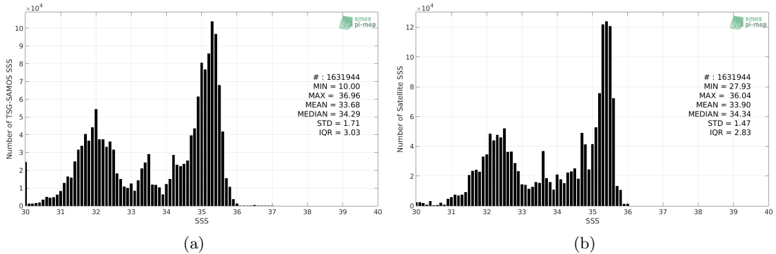
Figure 2: Histograms of SSS from TSG-SAMOS (a) and Aquarius-L3-JPL-V5-MONTHLY (b) considering all match-up pairs per bins of 0.1 over the Pacific Ocean Pi-MEP region and for the full satellite product period.
