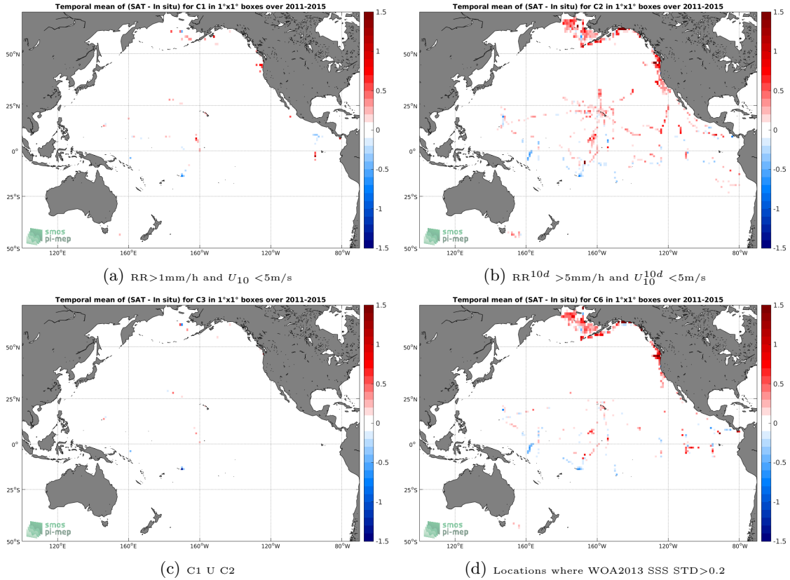
Figure 12: Temporal mean gridded over spatial boxes of size 1^\circ \times 1^\circ of \Delta SSS (Aquarius-L3-JPL-V5-MONTHLY - TSG-SAMOS) for 4 different subdatasets corresponding to: RR > 1\text{mm/h} and U_{10} < 5\text{m/s} (a), RR^{10d} > 5\text{mm/h} and U_{10}^{10d} < 5\text{m/s} (b), C1 U C2 (c), Locations where WOA2013 SSS STD > 0.2 (d).
