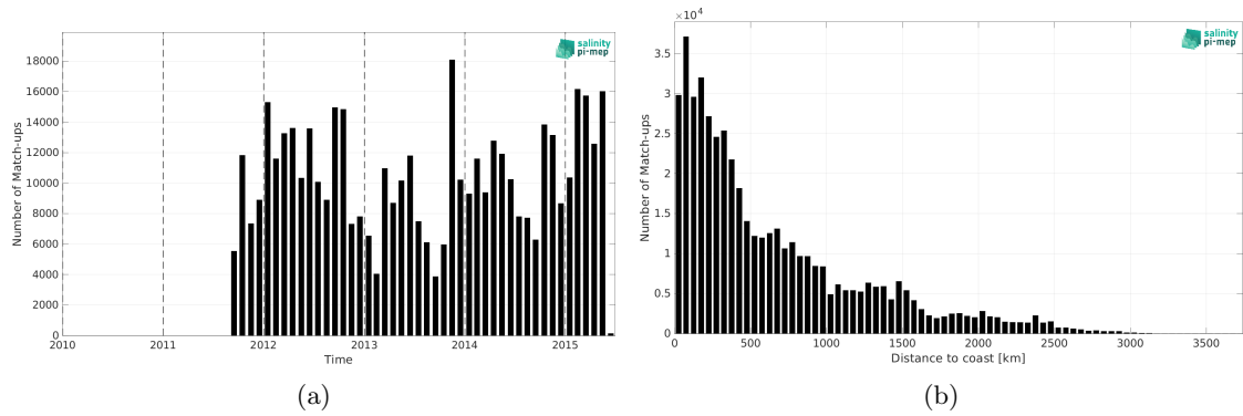
Figure 2: Number of match-ups between TSG (LEGOS-DM) and Aquarius SSS L3 CAP v5 - Monthly (JPL) SSS as a function of time (a) and as function of the distance to coast (b) over the Pacific Ocean Pi-MEP region and for the full satellite product period.
