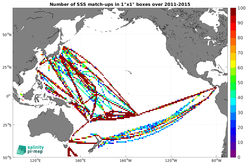
Figure 5: Number of SSS match-ups between TSG (LEGOS-DM) SSS and the Aquarius SSS L3 CAP v5 - Monthly (JPL) SSS product for the Pacific Ocean Pi-MEP region over 1^\circ \times 1^\circ boxes and for the full satellite product period.
