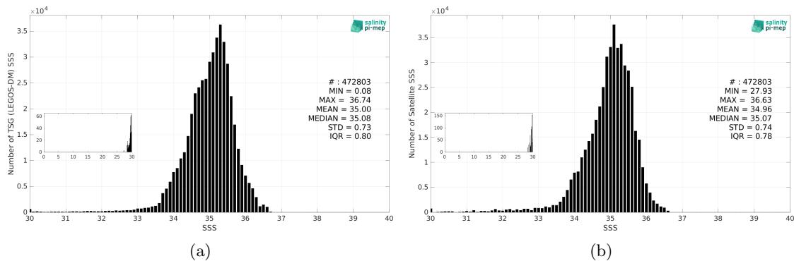
Figure 3: Histograms of SSS from TSG (LEGOS-DM) (a) and Aquarius SSS L3 CAP v5 - Monthly (JPL) (b) considering all match-up pairs per bins of 0.1 over the Pacific Ocean Pi-MEP region and for the full satellite product period.
