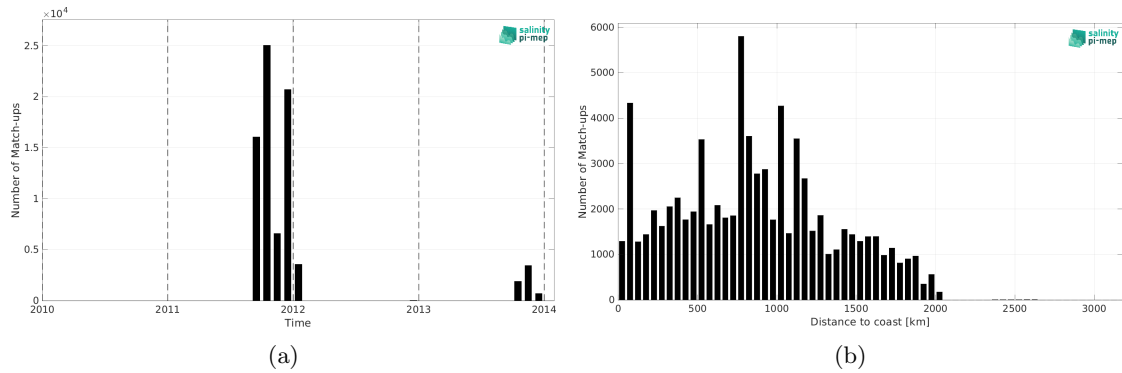
Figure 1: Number of match-ups between TSG (GOSUD-Sailing-ship) and Aquarius SSS L3 CAP v5 - Monthly (JPL) SSS as a function of time (a) and as function of the distance to coast (b) over the Pacific Ocean Pi-MEP region and for the full satellite product period.
