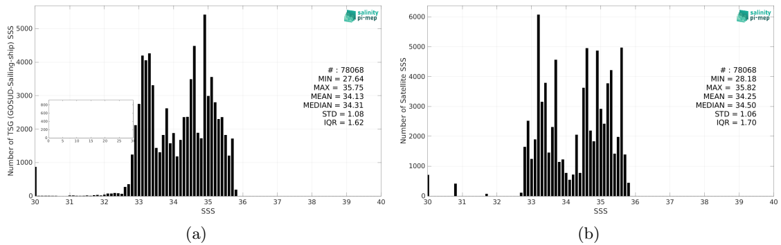
Figure 2: Histograms of SSS from TSG (GOSUD-Sailing-ship) (a) and Aquarius SSS L3 CAP v5 - Monthly (JPL) (b) considering all match-up pairs per bins of 0.1 over the Pacific Ocean Pi-MEP region and for the full satellite product period.
