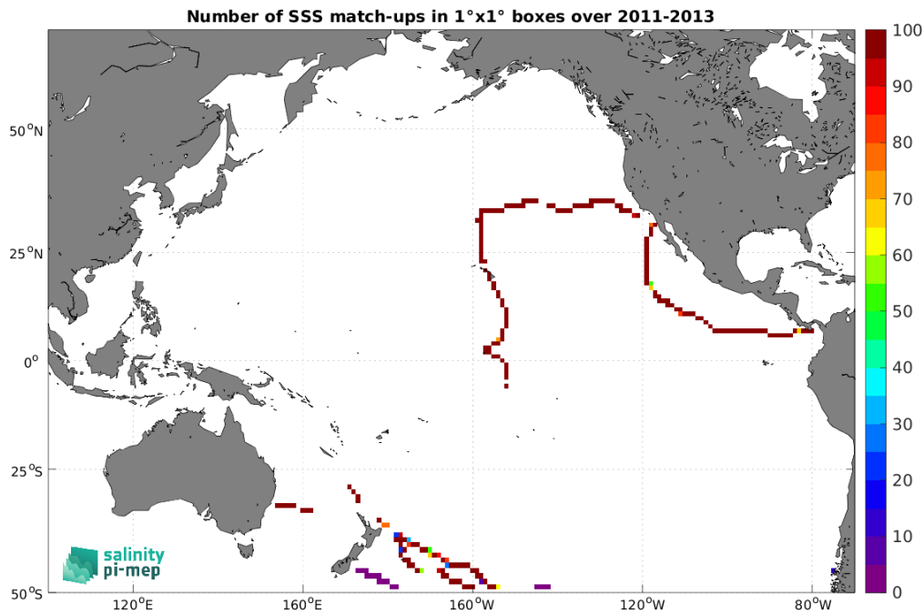
Figure 4: Number of SSS match-ups between TSG (GOSUD-Sailing-ship) SSS and the Aquarius SSS L3 CAP v5 - Monthly (JPL) SSS product for the Pacific Ocean Pi-MEP region over 1^\circ \times 1^\circ boxes and for the full satellite product period.
