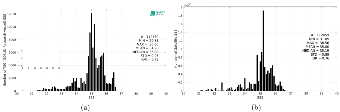
Figure 3: Histograms of SSS from TSG (GOSUD-Research-vessel) (a) and Aquarius SSS L3 CAP v5 - Monthly (JPL) (b) considering all match-up pairs per bins of 0.1 over the Pacific Ocean Pi-MEP region and for the full satellite product period.
