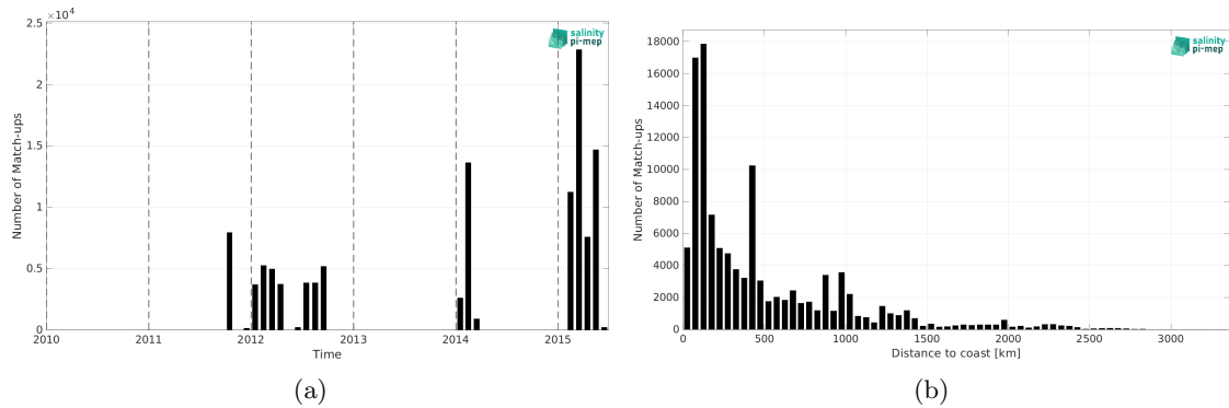
Figure 2: Number of match-ups between TSG (GOSUD-Research-vessel) and Aquarius SSS L3 CAP v5 - Monthly (JPL) SSS as a function of time (a) and as function of the distance to coast (b) over the Pacific Ocean Pi-MEP region and for the full satellite product period.
