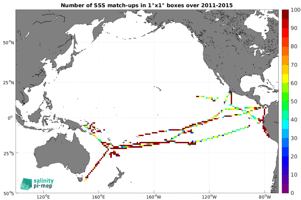
Figure 5: Number of SSS match-ups between TSG (GOSUD-Research-vessel) SSS and the Aquarius SSS L3 CAP v5 - Monthly (JPL) SSS product for the Pacific Ocean Pi-MEP region over 1^\circ \times 1^\circ boxes and for the full satellite product period.
