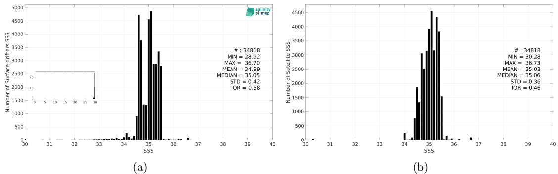
Figure 3: Histograms of SSS from Surface drifters (a) and Aquarius SSS L3 CAP v5 - Monthly (JPL) (b) considering all match-up pairs per bins of 0.1 over the Pacific Ocean Pi-MEP region and for the full satellite product period.
