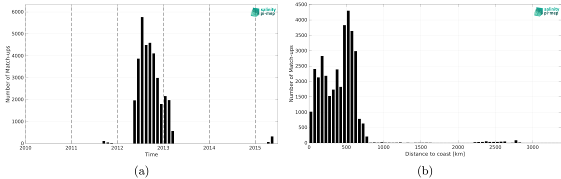
Figure 2: Number of match-ups between Surface drifters and Aquarius SSS L3 CAP v5 - Monthly (JPL) SSS as a function of time (a) and as function of the distance to coast (b) over the Pacific Ocean Pi-MEP region and for the full satellite product period.
