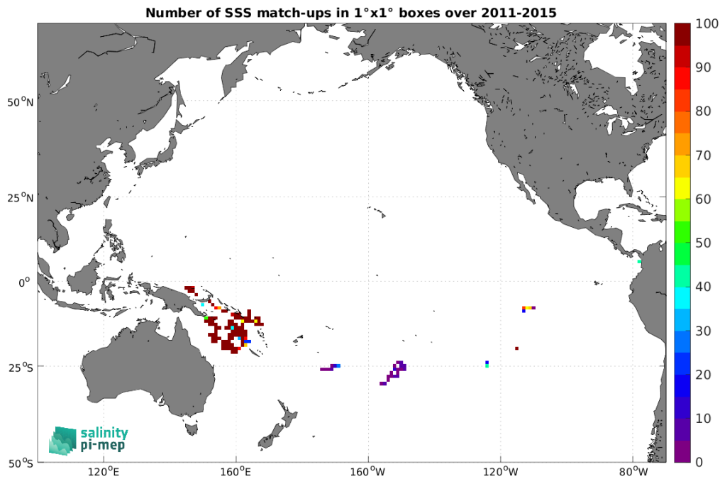
Figure 4: Number of SSS match-ups between Surface drifters SSS and the Aquarius SSS L3 CAP v5 - Monthly (JPL) SSS product for the Pacific Ocean Pi-MEP region over 1^\circ \times 1^\circ boxes and for the full satellite product period.
