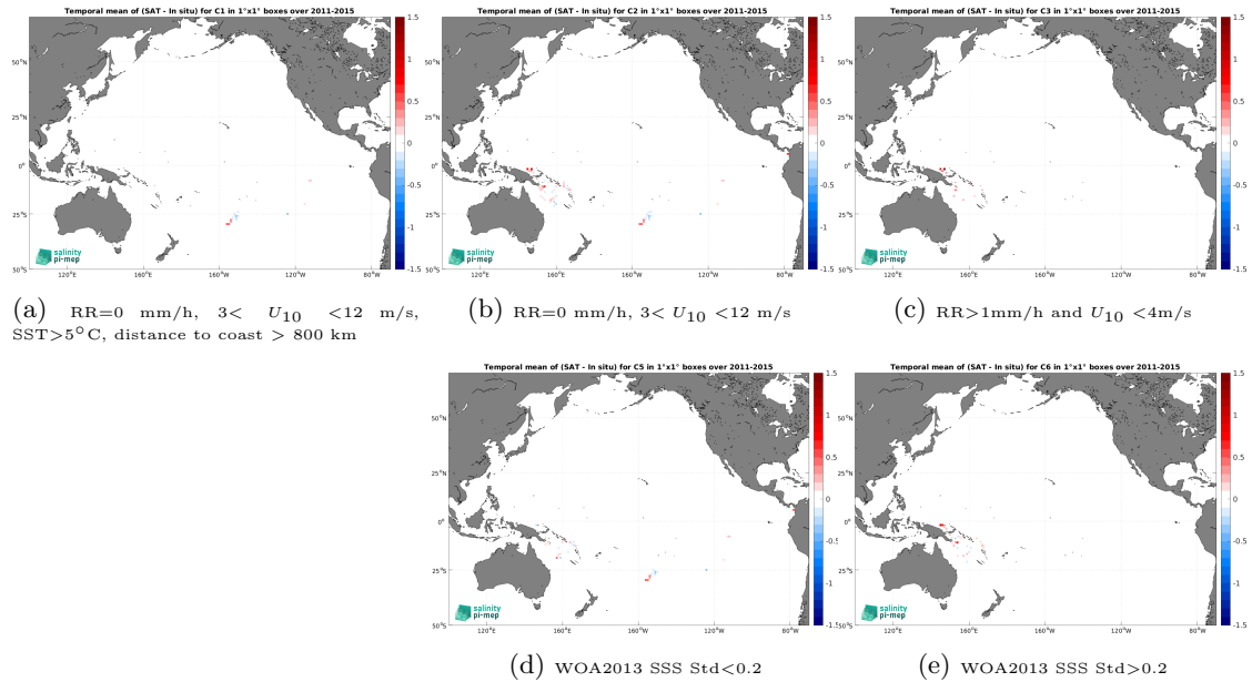
Figure 13: Temporal mean gridded over spatial boxes of size 1^\circ \times 1^\circ of \Delta\text{SSS} (Aquarius SSS L3 CAP v5 - Monthly (JPL) - Surface drifters) for 5 different subdatasets corresponding to:RR=0 mm/h, 3 < U_{10} < 12 m/s, SST >5^\circ\text{C} , distance to coast > 800 km (a), RR=0 mm/h, 3 < U_{10} < 12 m/s (b), RR >1 mm/h and U_{10} < 4 m/s (c), WOA2013 SSS Std <0.2 (d), WOA2013 SSS Std >0.2 (e).
