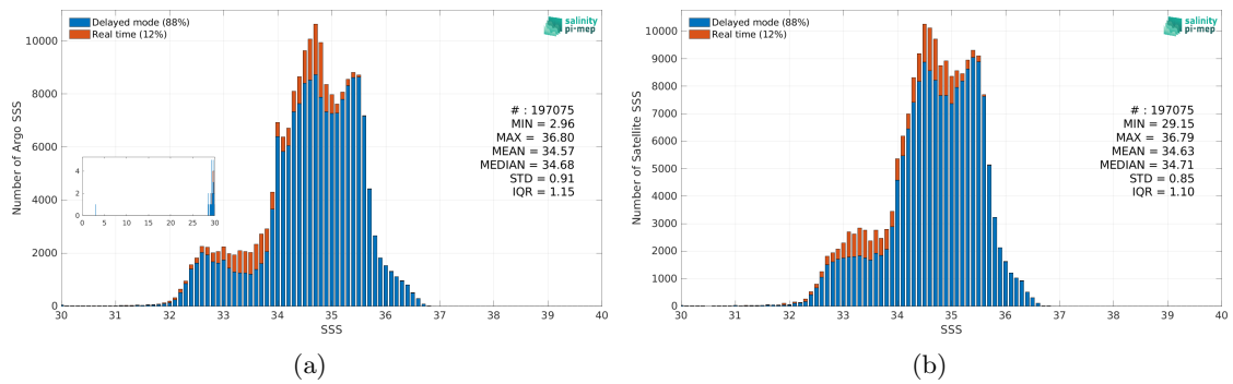
Figure 2: Histograms of SSS from Argo (a) and Aquarius SSS L3 CAP v5 - Monthly (JPL) (b) considering all match-up pairs per bins of 0.1 over the Pacific Ocean Pi-MEP region and for the full satellite product period.
