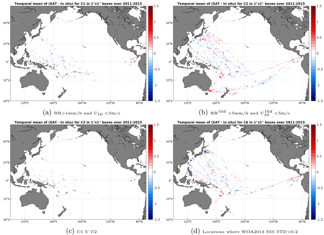
Figure 12: Temporal mean gridded over spatial boxes of size 1^\circ \times 1^\circ of \Delta SSS (Aquarius-L3-JPL-V4-7DAY-RUNNING - TSG-LEGOS-DM) for 4 different subdatasets corresponding to: RR > 1 mm/h and U_{10} < 5 m/s (a), RR 10d > 5 mm/h and U_{10}^{10d} < 5 m/s (b), C1 U C2 (c), Locations where WOA2013 SSS STD > 0.2 (d).
