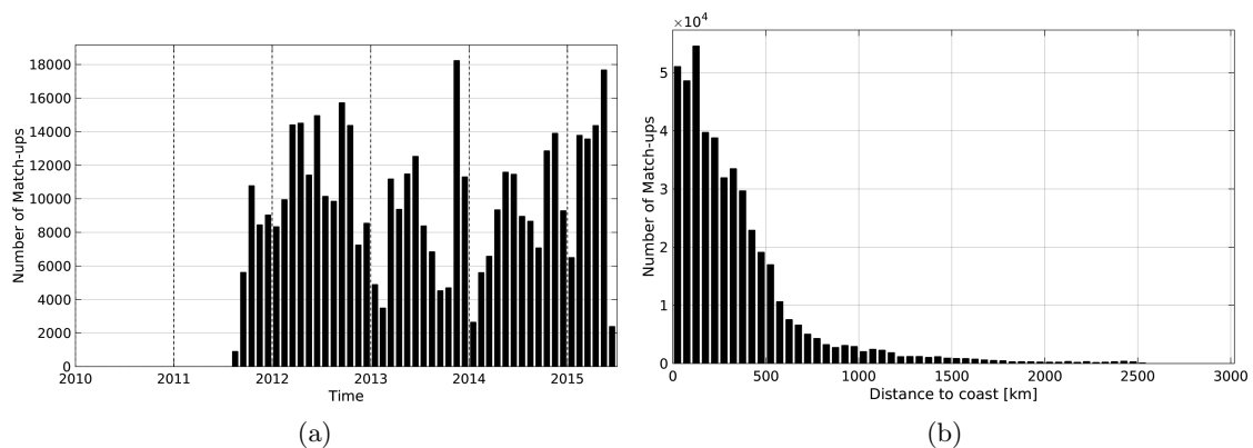
Figure 1: Number of match-ups between TSG-LEGOS-DM and Aquarius-L3-JPL-V4-7DAY-RUNNING SSS as a function of time (a) and as function of the distance to coast (b) over the Pacific Ocean Pi-MEP region and for the full satellite product period.
