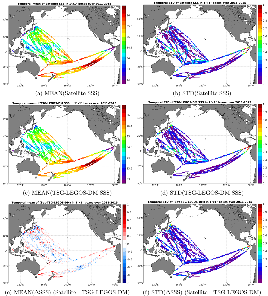
Figure 6: Temporal mean (left) and STD (right) of SSS from Aquarius-L3-JPL-V4-7DAY-RUNNING (top), TSG-LEGOS-DM (middle), and of \Delta SSS (Satellite - TSG-LEGOS-DM). Only match-up pairs are used to generate these maps.
