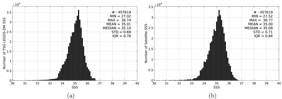
Figure 2: Histograms of SSS from TSG-LEGOS-DM (a) and Aquarius-L3-JPL-V4-7DAY-RUNNING (b) considering all match-up pairs per bins of 0.1 over the Pacific Ocean Pi-MEP region and for the full satellite product period.
