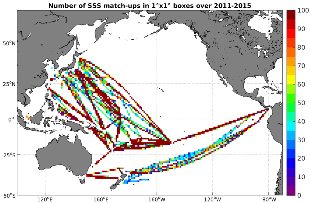
Figure 4: Number of SSS match-ups between TSG-LEGOS-DM SSS and the Aquarius-L3-JPL-V4-7DAY-RUNNING SSS product for the Pacific Ocean Pi-MEP region over 1^\circ \times 1^\circ boxes and for the full satellite product period.
