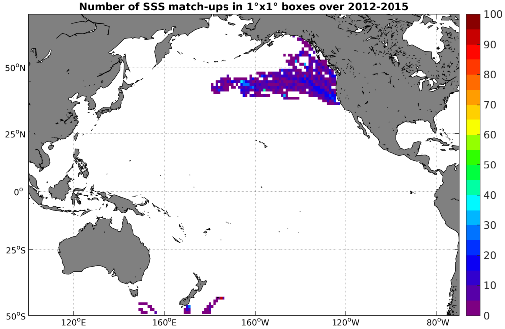
Figure 4: Number of SSS match-ups between Sea mammals SSS and the Aquarius-L3-JPL-V4-7DAY-RUNNING SSS product for the Pacific Ocean Pi-MEP region over 1^\circ \times 1^\circ boxes and for the full satellite product period.
