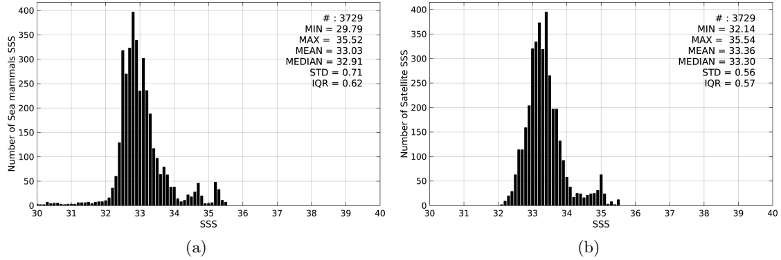
Figure 2: Histograms of SSS from Sea mammals (a) and Aquarius-L3-JPL-V4-7DAY-RUNNING (b) considering all match-up pairs per bins of 0.1 over the Pacific Ocean Pi-MEP region and for the full satellite product period.
