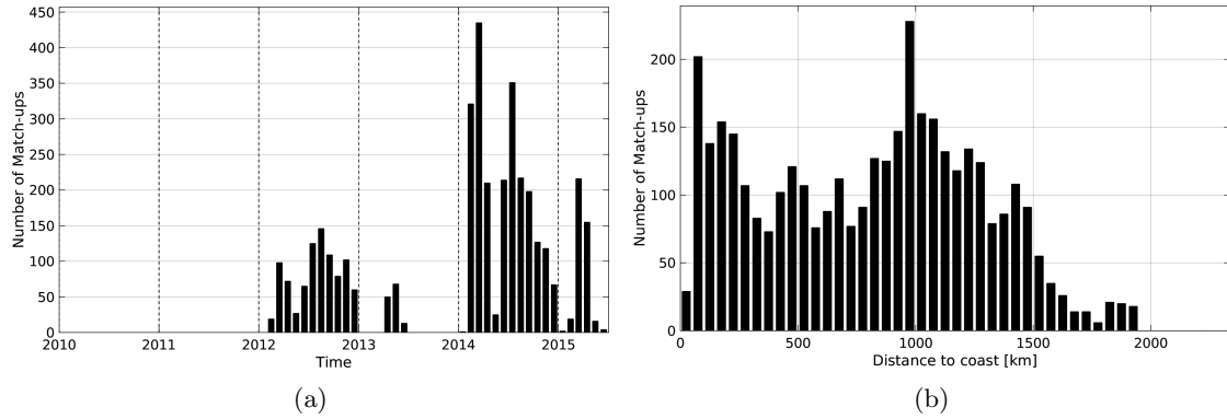
Figure 1: Number of match-ups between Sea mammals and Aquarius-L3-JPL-V4-7DAY-RUNNING SSS as a function of time (a) and as function of the distance to coast (b) over the Pacific Ocean Pi-MEP region and for the full satellite product period.
