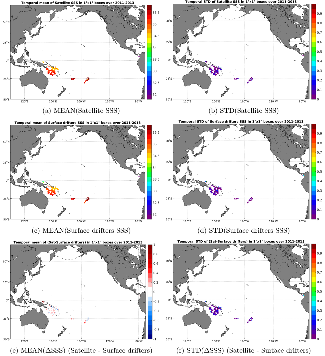
Figure 5: Temporal mean (left) and STD (right) of SSS from Aquarius-L3-JPL-V4-7DAY-RUNNING (top), Surface drifters (middle), and of \Delta SSS (Satellite - Surface drifters). Only match-up pairs are used to generate these maps.
