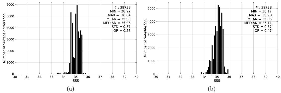
Figure 2: Histograms of SSS from Surface drifters (a) and Aquarius-L3-JPL-V4-7DAY-RUNNING (b) considering all match-up pairs per bins of 0.1 over the Pacific Ocean Pi-MEP region and for the full satellite product period.
