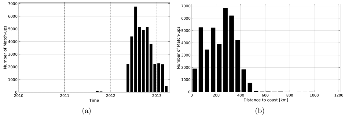
Figure 1: Number of match-ups between Surface drifters and Aquarius-L3-JPL-V4-7DAY-RUNNING SSS as a function of time (a) and as function of the distance to coast (b) over the Pacific Ocean Pi-MEP region and for the full satellite product period.
