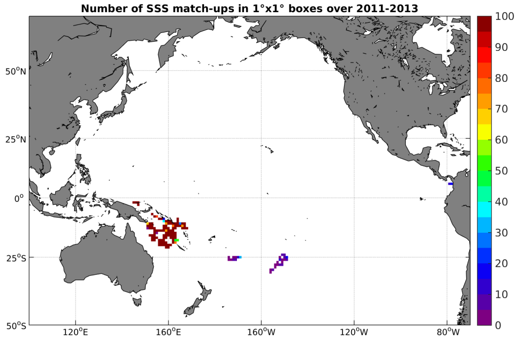
Figure 3: Number of SSS match-ups between Surface drifters SSS and the Aquarius-L3-JPL-V4-7DAY-RUNNING SSS product for the Pacific Ocean Pi-MEP region over 1^\circ \times 1^\circ boxes and for the full satellite product period.
