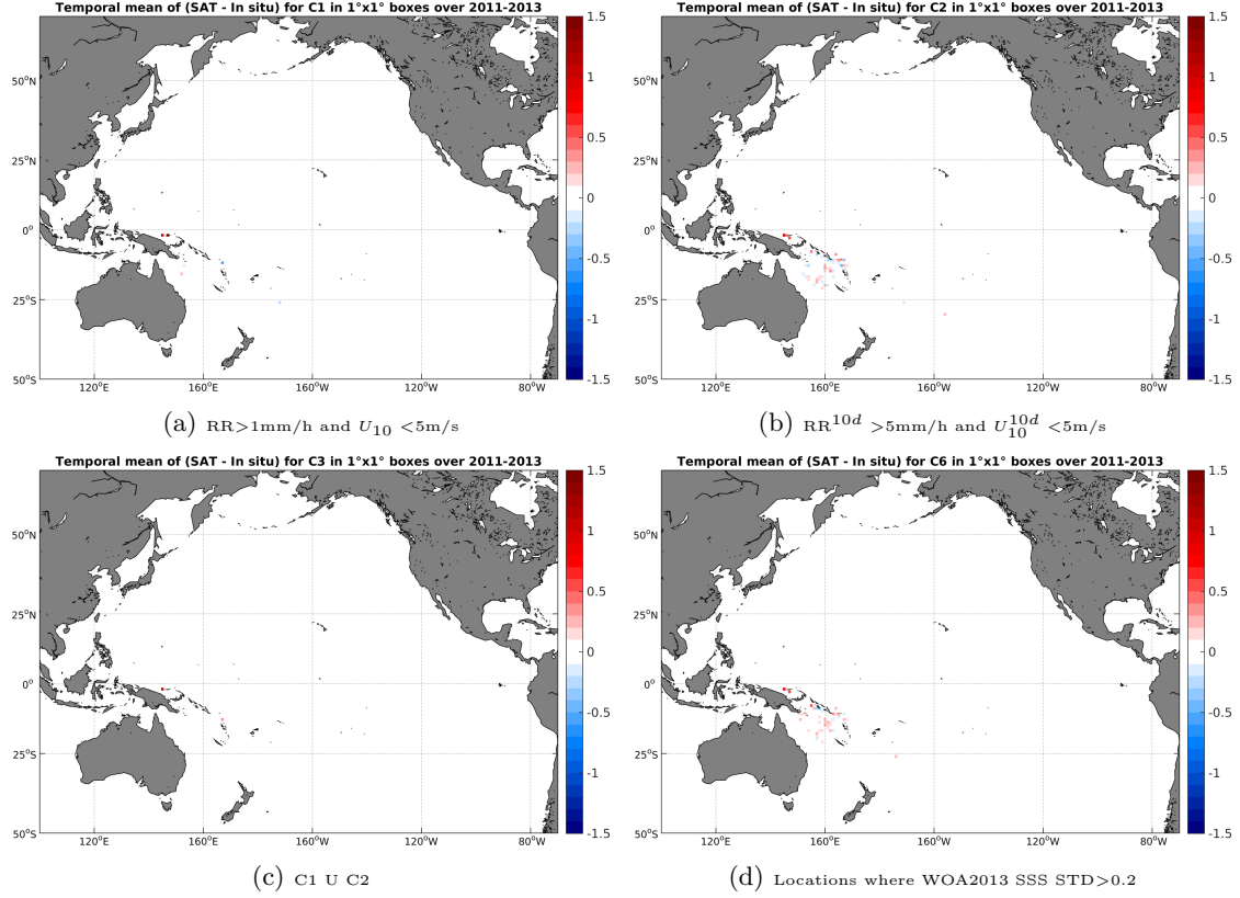
Figure 11: Temporal mean gridded over spatial boxes of size 1^\circ \times 1^\circ of \Delta SSS (Aquarius-L3-JPL-V4-7DAY-RUNNING - Surface drifters) for 4 different subdatasets corresponding to: RR > 1mm/h and U_{10} < 5 m/s (a), RR^{10d} > 5 mm/h and U_{10}^{10d} < 5 m/s (b), C1 U C2 (c), Locations where WOA2013 SSS STD > 0.2 (d).
