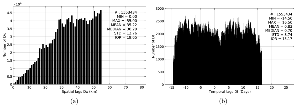
Figure 5: Histograms of the spatial (a) and temporal (b) lags between the time of the TSG-SAMOS measurements and the date of the corresponding Aquarius-L3-JPL-V4-MONTHLY SSS product.
