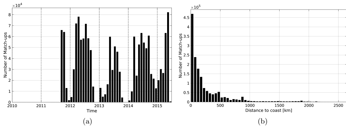
Figure 1: Number of match-ups between TSG-SAMOS and Aquarius-L3-JPL-V4-MONTHLY SSS as a function of time (a) and as function of the distance to coast (b) over the Pacific Ocean Pi-MEP region and for the full satellite product period.
