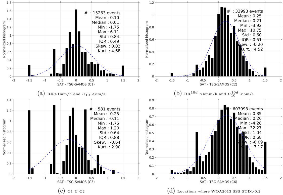
Figure 13: Normalized histogram of \Delta\text{SSS} (Aquarius-L3-JPL-V4-MONTHLY - TSG-SAMOS) for 6 different subdatasets corresponding to: \text{RR} > 1\text{mm/h} and U_{10} < 5\text{m/s} (a), \text{RR}^{10d} > 5\text{mm/h} and U_{10}^{10d} < 5\text{m/s} (b), C1 U C2 (c), Locations where WOA2013 SSS STD > 0.2 (d).
