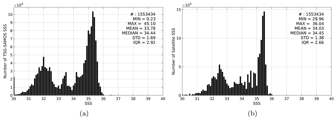
Figure 2: Histograms of SSS from TSG-SAMOS (a) and Aquarius-L3-JPL-V4-MONTHLY (b) considering all match-up pairs per bins of 0.1 over the Pacific Ocean Pi-MEP region and for the full satellite product period.
