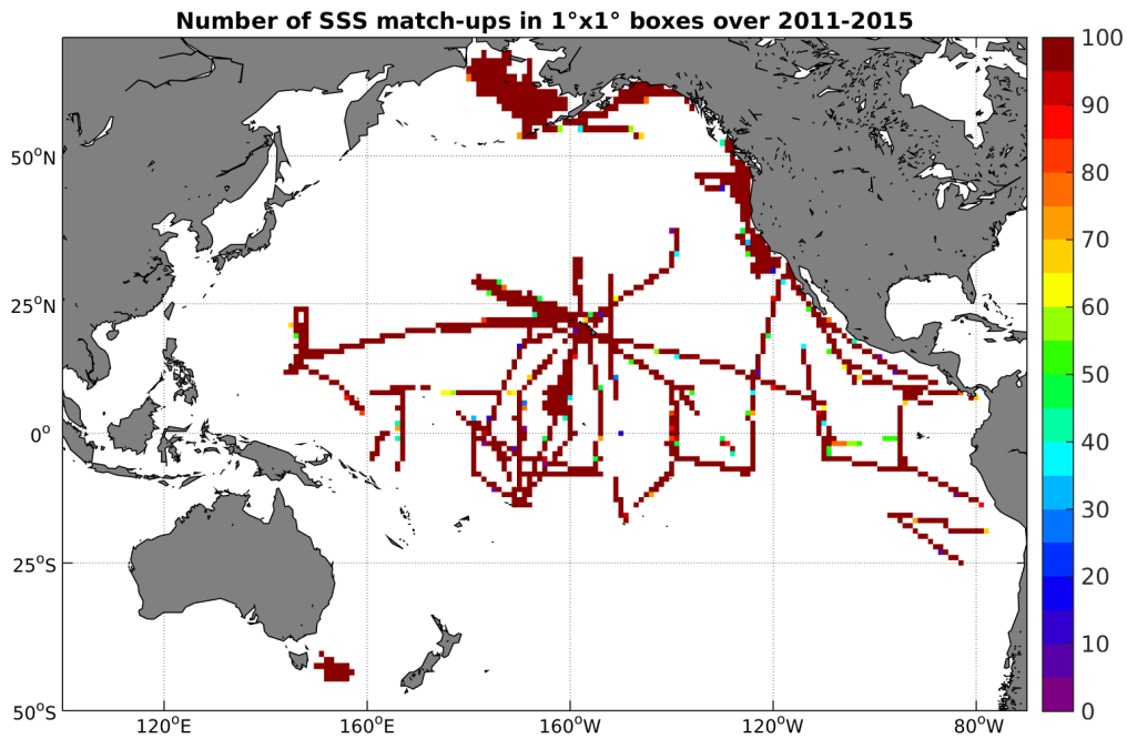
Figure 4: Number of SSS match-ups between TSG-SAMOS SSS and the Aquarius-L3-JPL-V4-MONTHLY SSS product for the Pacific Ocean Pi-MEP region over 1^\circ \times 1^\circ boxes and for the full satellite product period.
