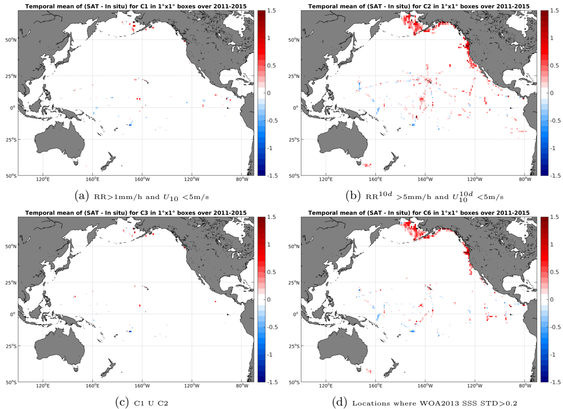
Figure 12: Temporal mean gridded over spatial boxes of size 1^\circ \times 1^\circ of \Delta SSS (Aquarius-L3-JPL-V4-MONTHLY - TSG-SAMOS) for 4 different subdatasets corresponding to:RR >1 mm/h and U_{10} < 5 m/s (a), RR 10d > 5 mm/h and U_{10}^{10d} < 5 m/s (b), C1 U C2 (c),Locations where WOA2013 SSS STD >0.2 (d).
