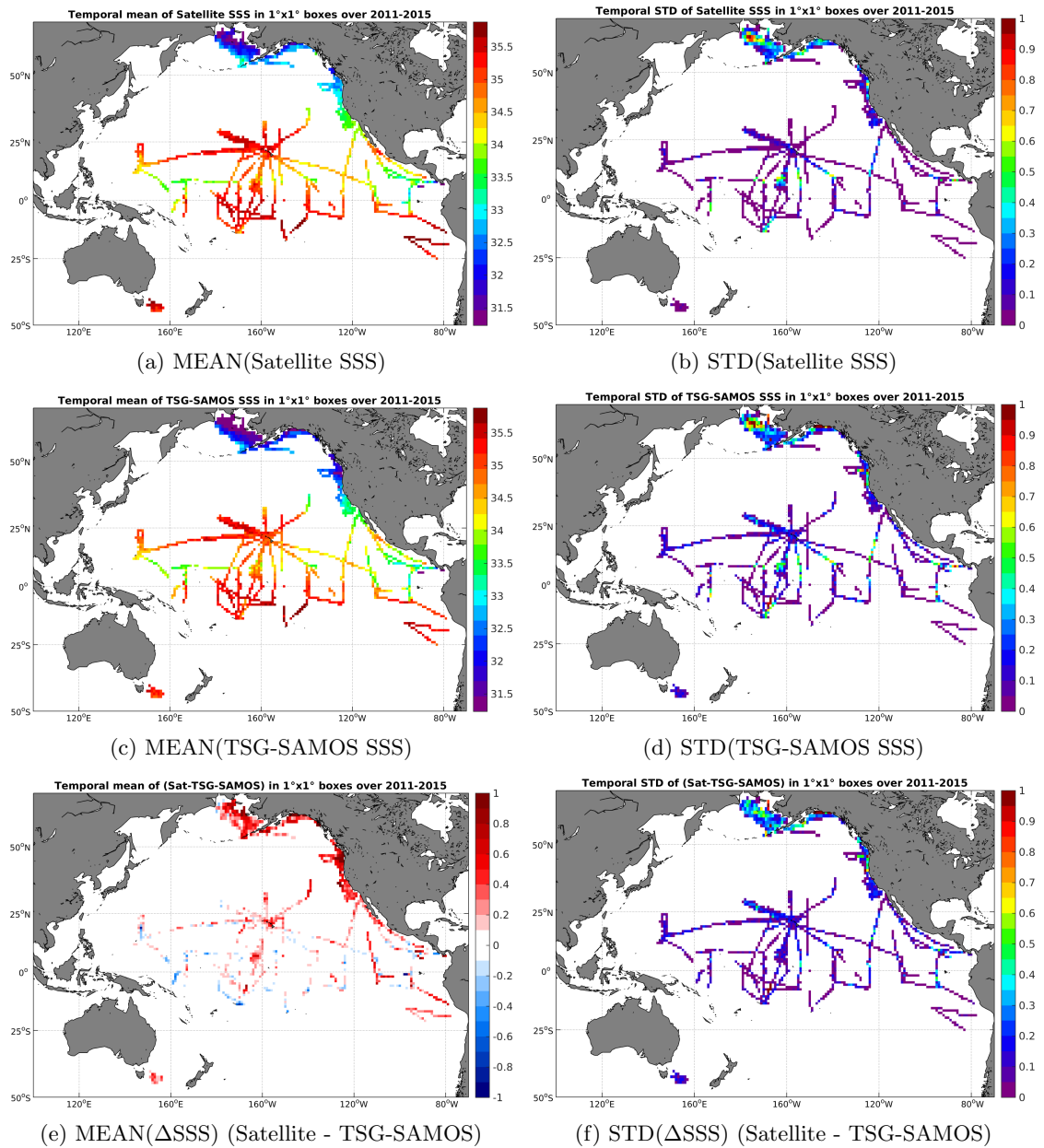
Figure 6: Temporal mean (left) and STD (right) of SSS from Aquarius-L3-JPL-V4-MONTHLY (top), TSG-SAMOS (middle), and of \Delta SSS (Satellite - TSG-SAMOS). Only match-up pairs are used to generate these maps.
