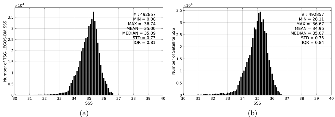
Figure 2: Histograms of SSS from TSG-LEGOS-DM (a) and Aquarius-L3-JPL-V4-MONTHLY (b) considering all match-up pairs per bins of 0.1 over the Pacific Ocean Pi-MEP region and for the full satellite product period.
