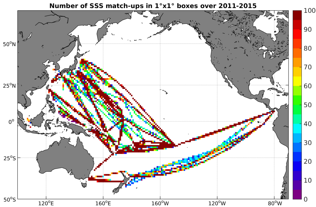
Figure 4: Number of SSS match-ups between TSG-LEGOS-DM SSS and the Aquarius-L3-JPL-V4-MONTHLY SSS product for the Pacific Ocean Pi-MEP region over 1^\circ \times 1^\circ boxes and for the full satellite product period.
