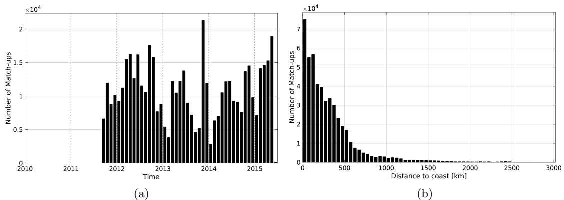
Figure 1: Number of match-ups between TSG-LEGOS-DM and Aquarius-L3-JPL-V4-MONTHLY SSS as a function of time (a) and as function of the distance to coast (b) over the Pacific Ocean Pi-MEP region and for the full satellite product period.
