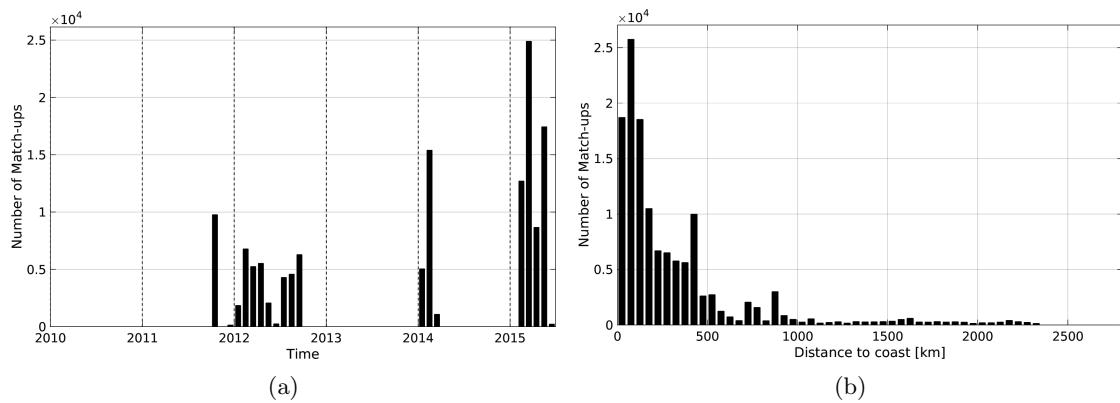
Figure 1: Number of match-ups between TSG-GOSUD-Research-vessel and Aquarius-L3-JPL-V4-MONTHLY SSS as a function of time (a) and as function of the distance to coast (b) over the Pacific Ocean Pi-MEP region and for the full satellite product period.
