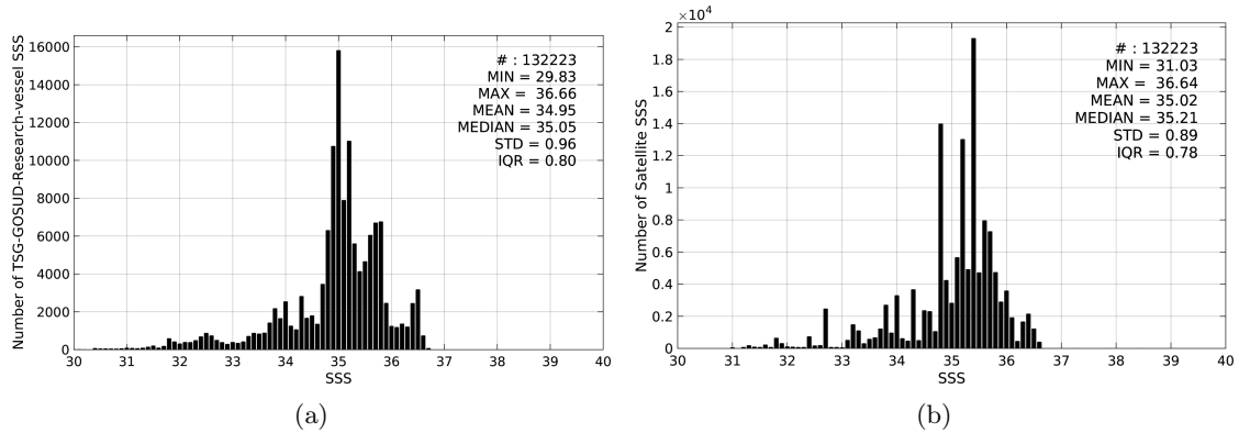
Figure 2: Histograms of SSS from TSG-GOSUD-Research-vessel (a) and Aquarius-L3-JPL-V4-MONTHLY (b) considering all match-up pairs per bins of 0.1 over the Pacific Ocean Pi-MEP region and for the full satellite product period.
