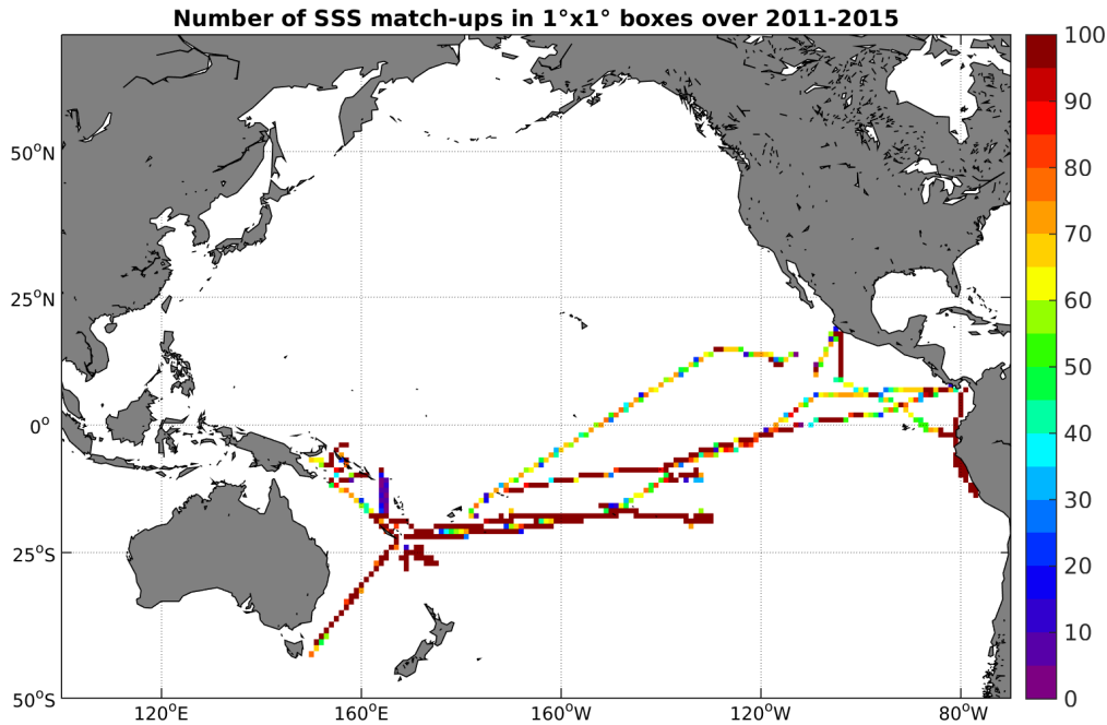
Figure 4: Number of SSS match-ups between TSG-GOSUD-Research-vessel SSS and the Aquarius-L3-JPL-V4-MONTHLY SSS product for the Pacific Ocean Pi-MEP region over 1^\circ \times 1^\circ boxes and for the full satellite product period.
