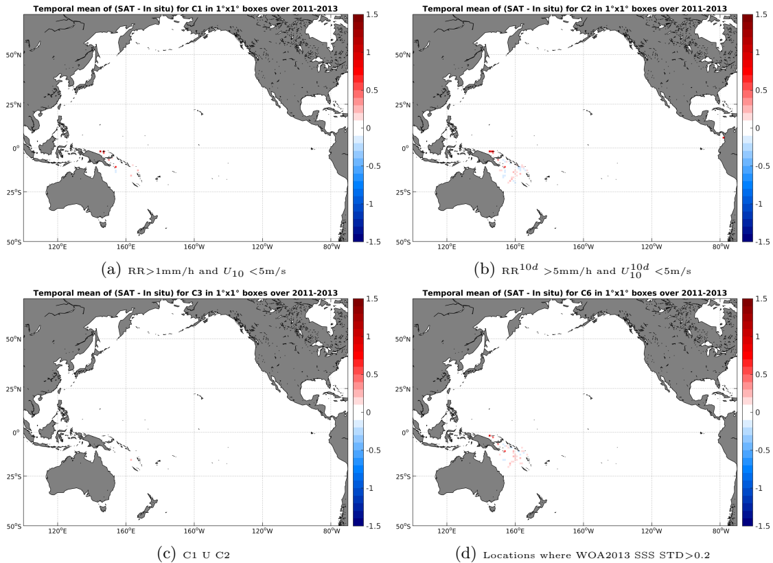
Figure 11: Temporal mean gridded over spatial boxes of size 1^\circ \times 1^\circ of \Delta SSS (Aquarius-L3-JPL-V4-MONTHLY - Surface drifters) for 4 different subdatasets corresponding to: RR > 1\text{mm/h} and U_{10} < 5\text{m/s} (a), RR^{10d} > 5\text{mm/h} and U_{10}^{10d} < 5\text{m/s} (b), C1 U C2 (c), Locations where WOA2013 SSS STD > 0.2 (d).
