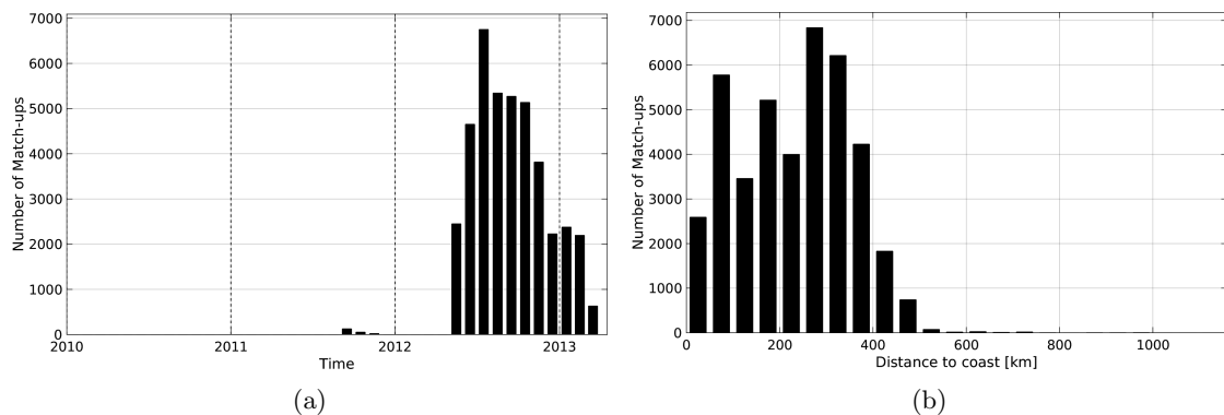
Figure 1: Number of match-ups between Surface drifters and Aquarius-L3-JPL-V4-MONTHLY SSS as a function of time (a) and as function of the distance to coast (b) over the Pacific Ocean Pi-MEP region and for the full satellite product period.
