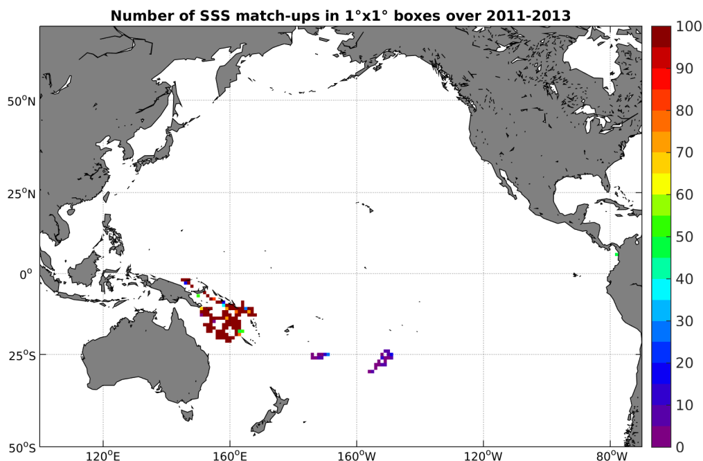
Figure 3: Number of SSS match-ups between Surface drifters SSS and the Aquarius-L3-JPL-V4-MONTHLY SSS product for the Pacific Ocean Pi-MEP region over 1^\circ \times 1^\circ boxes and for the full satellite product period.
