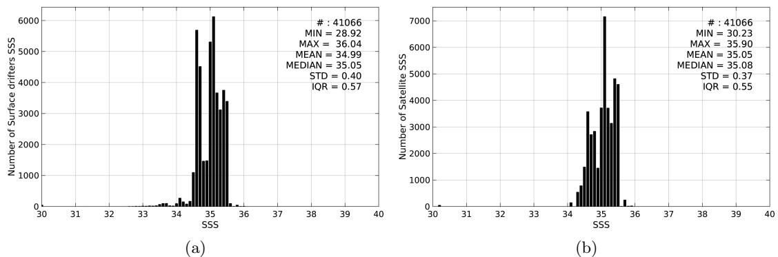
Figure 2: Histograms of SSS from Surface drifters (a) and Aquarius-L3-JPL-V4-MONTHLY (b) considering all match-up pairs per bins of 0.1 over the Pacific Ocean Pi-MEP region and for the full satellite product period.
