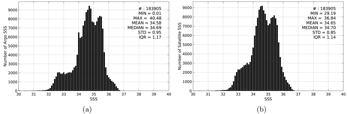
Figure 2: Histograms of SSS from Argo (a) and Aquarius-L3-JPL-V4-MONTHLY (b) considering all match-up pairs per bins of 0.1 over the Pacific Ocean Pi-MEP region and for the full satellite product period.
