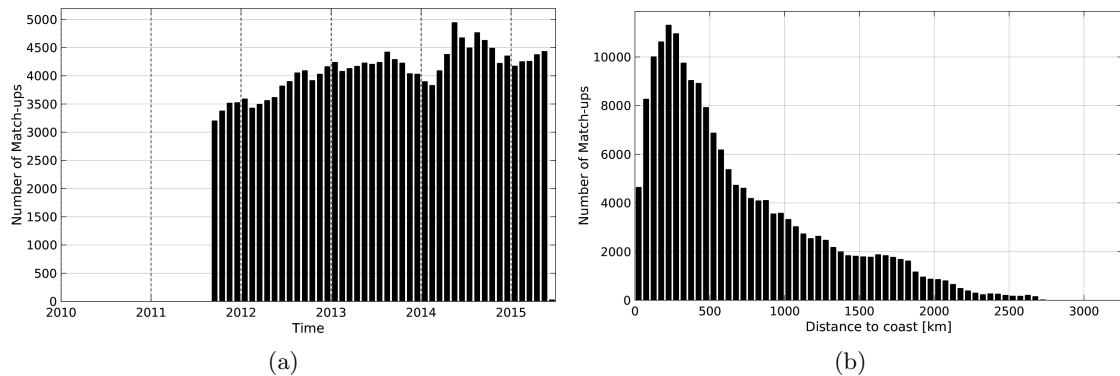
Figure 1: Number of match-ups between Argo and Aquarius-L3-JPL-V4-MONTHLY SSS as a function of time (a) and as function of the distance to coast (b) over the Pacific Ocean Pi-MEP region and for the full satellite product period.
