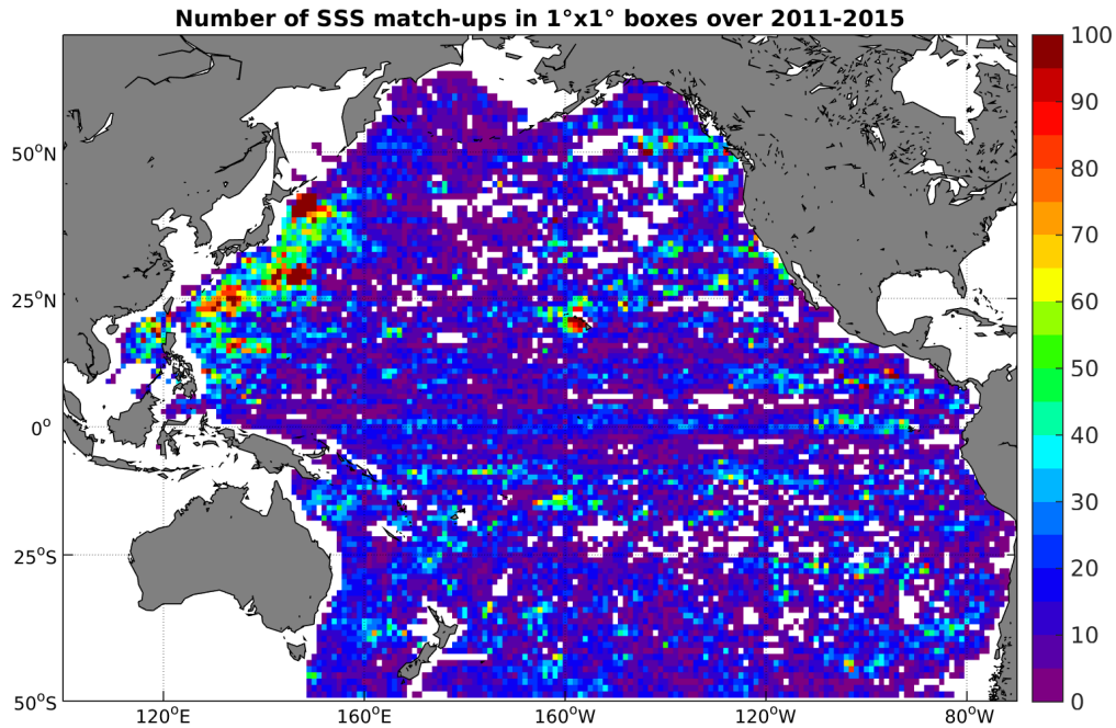
Figure 4: Number of SSS match-ups between Argo SSS and the Aquarius-L3-JPL-V4-MONTHLY SSS product for the Pacific Ocean Pi-MEP region over 1°x1° boxes and for the full satellite product period.
