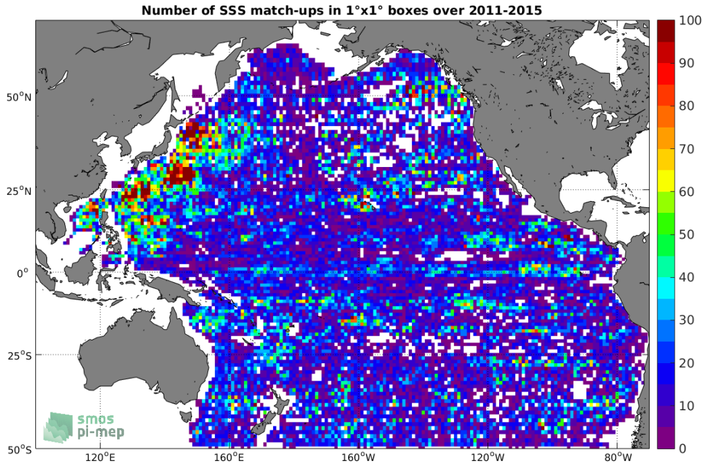
Figure 4: Number of SSS match-ups between Argo SSS and the Aquarius SSS L2-AVERAGED OR v5 (NASA-GSFC) SSS product for the Pacific Ocean Pi-MEP region over 1^\circ \times 1^\circ boxes and for the full satellite product period.
