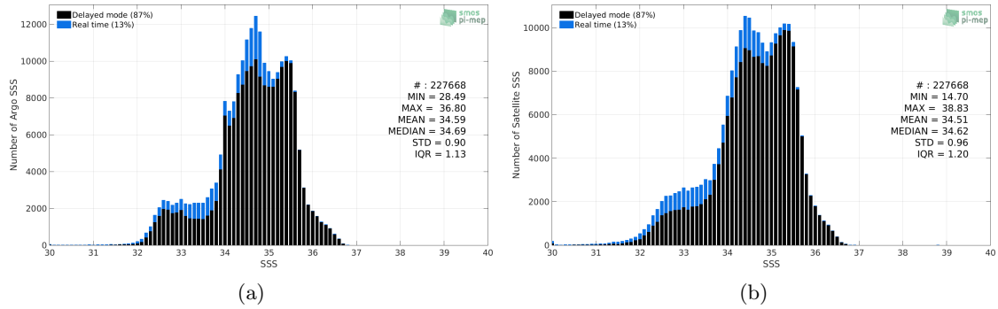
Figure 2: Histograms of SSS from Argo (a) and Aquarius SSS L2-AVERAGED OR v5 (NASA-GSFC) (b) considering all match-up pairs per bins of 0.1 over the Pacific Ocean Pi-MEP region and for the full satellite product period.
