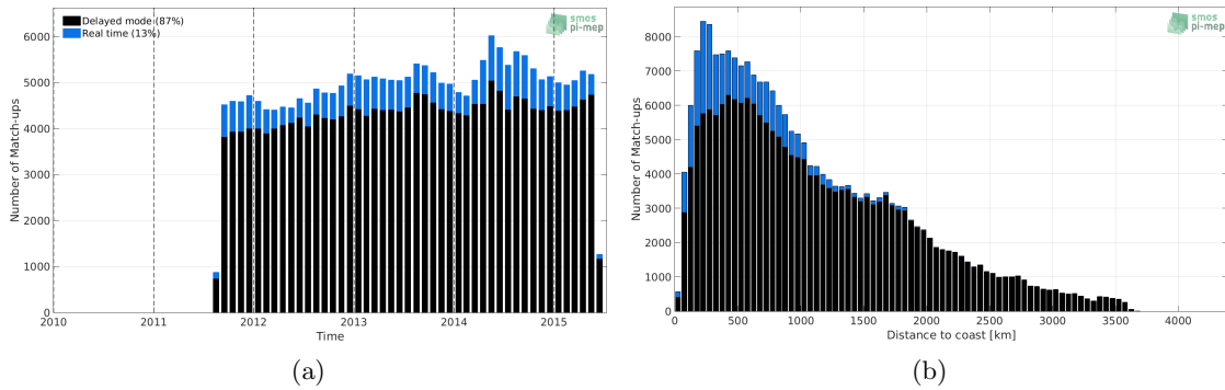
Figure 1: Number of match-ups between Argo and Aquarius SSS L2-AVERAGED OR v5 (NASA-GSFC) SSS as a function of time (a) and as function of the distance to coast (b) over the Pacific Ocean Pi-MEP region and for the full satellite product period.
