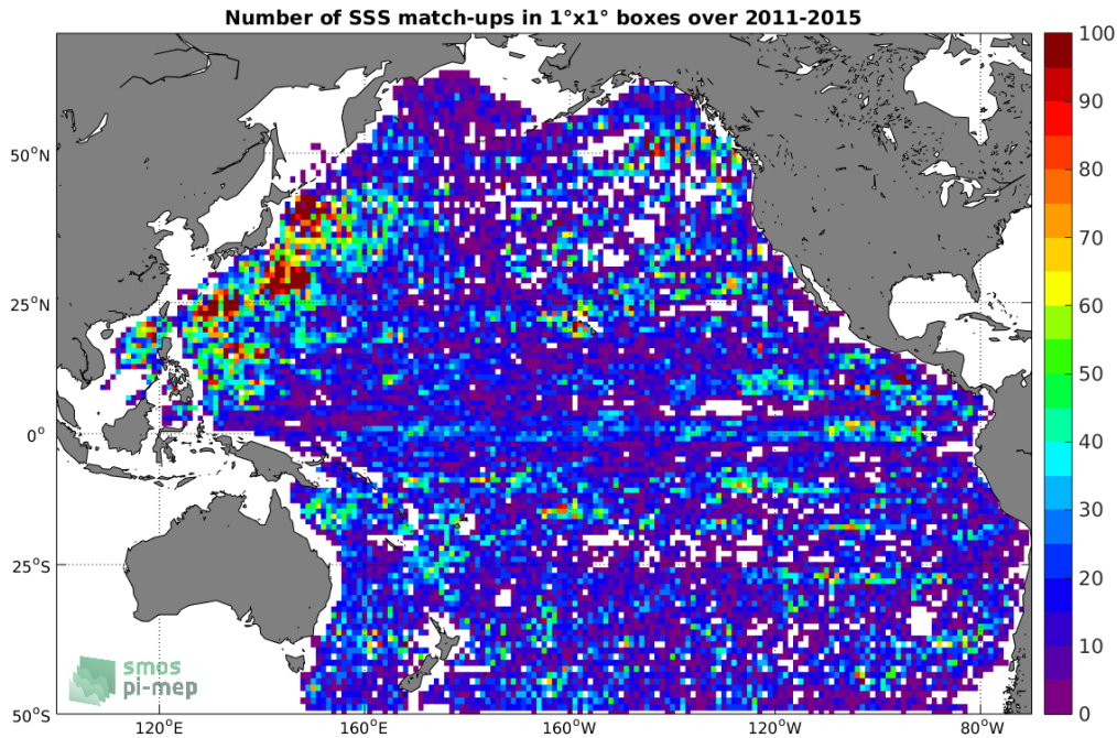
Figure 4: Number of SSS match-ups between Argo SSS and the Aquarius SSS L2-AVERAGED CAP v5 (JPL) SSS product for the Pacific Ocean Pi-MEP region over 1^\circ \times 1^\circ boxes and for the full satellite product period.
