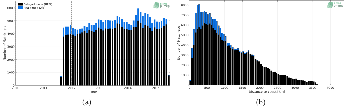
Figure 1: Number of match-ups between Argo and Aquarius SSS L2-AVERAGED CAP v5 (JPL) SSS as a function of time (a) and as function of the distance to coast (b) over the Pacific Ocean Pi-MEP region and for the full satellite product period.
