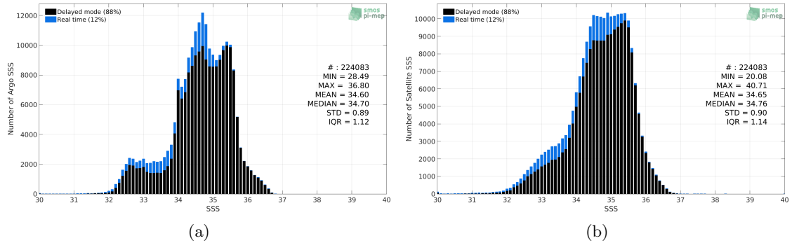
Figure 2: Histograms of SSS from Argo (a) and Aquarius SSS L2-AVERAGED CAP v5 (JPL) (b) considering all match-up pairs per bins of 0.1 over the Pacific Ocean Pi-MEP region and for the full satellite product period.
