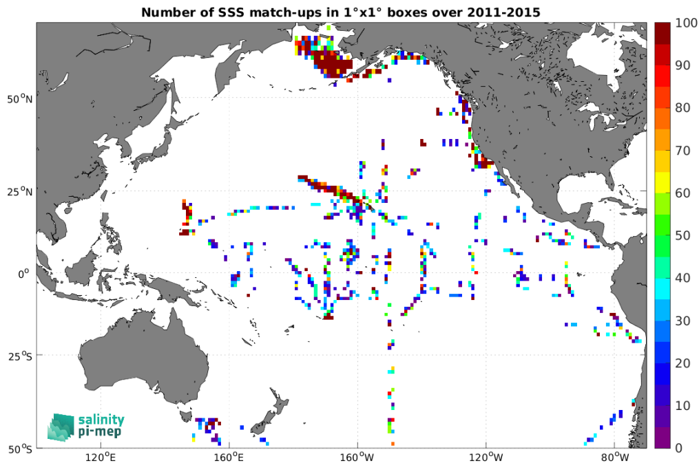
Figure 4: Number of SSS match-ups between TSG (SAMOS) SSS and the Aquarius SSS L2 OR v5 (NASA-GSFC) SSS product for the Pacific Ocean Pi-MEP region over 1^\circ \times 1^\circ boxes and for the full satellite product period.
