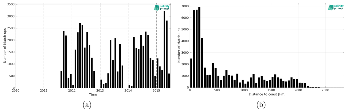
Figure 1: Number of match-ups between TSG (SAMOS) and Aquarius SSS L2 OR v5 (NASA-GSFC) SSS as a function of time (a) and as function of the distance to coast (b) over the Pacific Ocean Pi-MEP region and for the full satellite product period.
