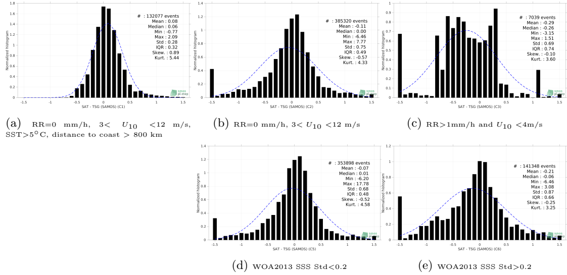
Figure 13: Normalized histogram of \Delta\text{SSS} (Aquarius SSS L2 OR v5 (NASA-GSFC) - TSG (SAMOS)) for 5 different subdatasets corresponding to: RR=0 mm/h, 3 < U_{10} < 12 m/s, SST>5°C, distance to coast > 800 km (a), RR=0 mm/h, 3 < U_{10} < 12 m/s (b), RR>1mm/h and U_{10} < 4 m/s (c), WOA2013 SSS Std<0.2 (d), WOA2013 SSS Std>0.2 (e).
