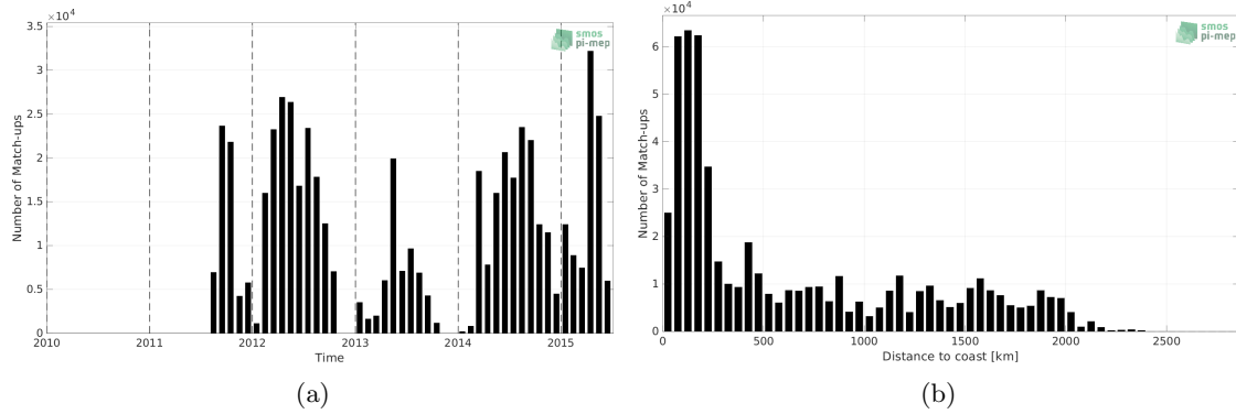
Figure 1: Number of match-ups between TSG (SAMOS) and Aquarius SSS L2 OR v5 (NASA-GSFC) SSS as a function of time (a) and as function of the distance to coast (b) over the Pacific Ocean Pi-MEP region and for the full satellite product period.
