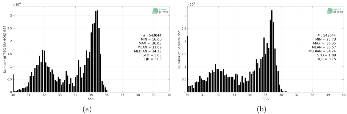
Figure 2: Histograms of SSS from TSG (SAMOS) (a) and Aquarius SSS L2 OR v5 (NASA-GSFC) (b) considering all match-up pairs per bins of 0.1 over the Pacific Ocean Pi-MEP region and for the full satellite product period.
