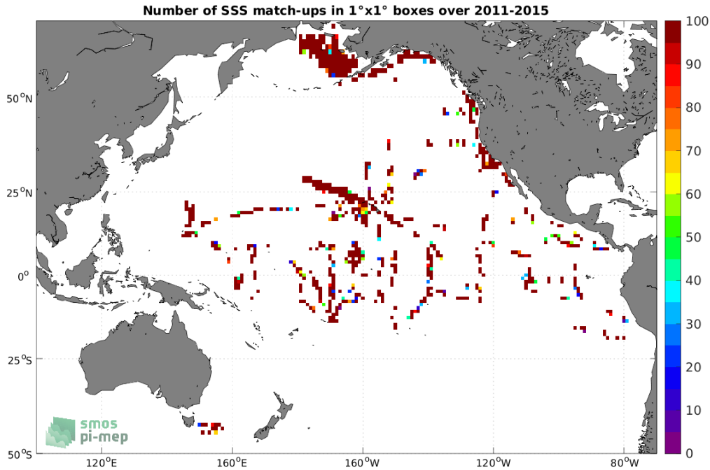
Figure 4: Number of SSS match-ups between TSG (SAMOS) SSS and the Aquarius SSS L2 OR v5 (NASA-GSFC) SSS product for the Pacific Ocean Pi-MEP region over 1°x1° boxes and for the full satellite product period.
