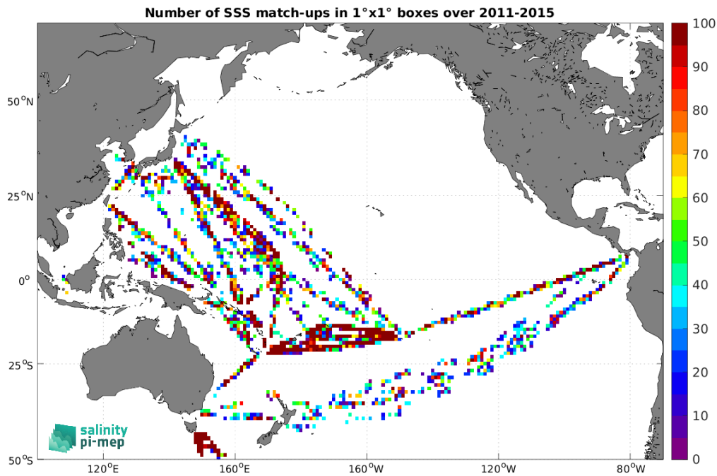
Figure 5: Number of SSS match-ups between TSG (LEGOS-DM) SSS and the Aquarius SSS L2 OR v5 (NASA-GSFC) SSS product for the Pacific Ocean Pi-MEP region over 1^\circ \times 1^\circ boxes and for the full satellite product period.
