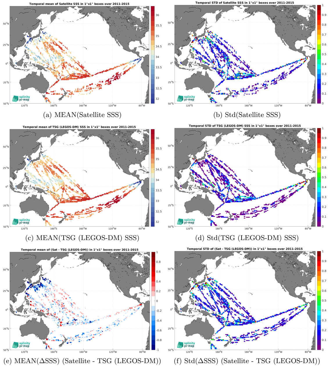
Figure 7: Temporal mean (left) and Std (right) of SSS from Aquarius SSS L2 OR v5 (NASA-GSFC) (top), TSG (LEGOS-DM) (middle), and of \Delta SSS (Satellite - TSG (LEGOS-DM)). Only match-up pairs are used to generate these maps.
