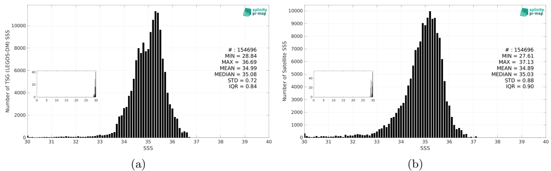
Figure 3: Histograms of SSS from TSG (LEGOS-DM) (a) and Aquarius SSS L2 OR v5 (NASA-GSFC) (b) considering all match-up pairs per bins of 0.1 over the Pacific Ocean Pi-MEP region and for the full satellite product period.
