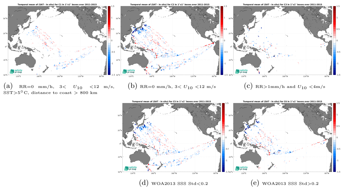
Figure 14: Temporal mean gridded over spatial boxes of size 1^\circ \times 1^\circ of \Delta SSS (Aquarius SSS L2 OR v5 (NASA-GSFC) - TSG (LEGOS-DM)) for 5 different subdatasets corresponding to:RR=0 mm/h, 3 < U_{10} < 12 m/s, SST > 5^\circ\text{C} , distance to coast > 800 km (a), RR=0 mm/h, 3 < U_{10} < 12 m/s (b), RR > 1 mm/h and U_{10} < 4 m/s (c), WOA2013 SSS Std < 0.2 (d), WOA2013 SSS Std > 0.2 (e).
