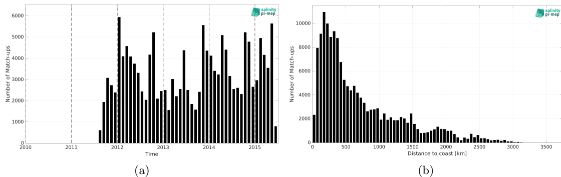
Figure 2: Number of match-ups between TSG (LEGOS-DM) and Aquarius SSS L2 OR v5 (NASA-GSFC) SSS as a function of time (a) and as function of the distance to coast (b) over the Pacific Ocean Pi-MEP region and for the full satellite product period.
