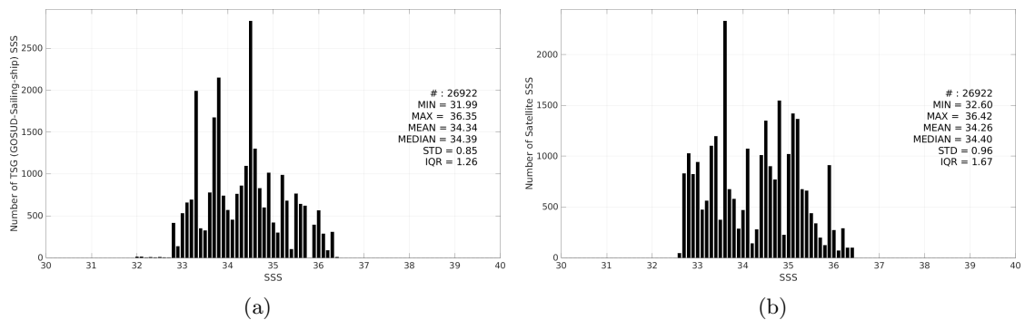
Figure 3: Histograms of SSS from TSG (GOSUD-Sailing-ship) (a) and Aquarius SSS L2 OR v5 (NASA-GSFC) (b) considering all match-up pairs per bins of 0.1 over the Pacific Ocean Pi-MEP region and for the full satellite product period.
