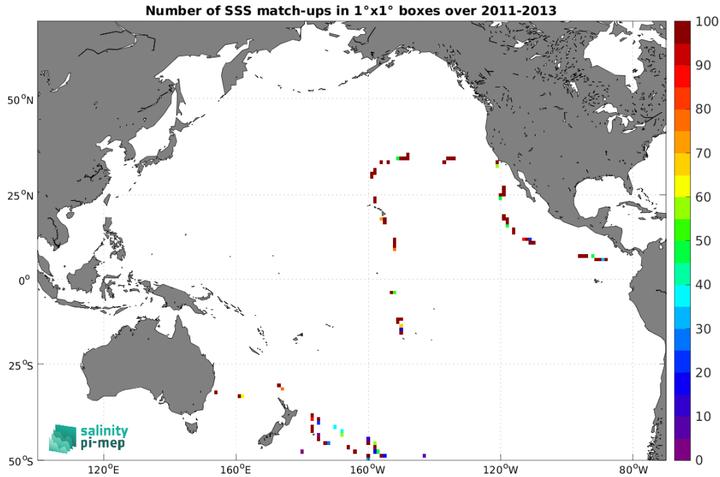
Figure 5: Number of SSS match-ups between TSG (GOSUD-Sailing-ship) SSS and the Aquarius SSS L2 OR v5 (NASA-GSFC) SSS product for the Pacific Ocean Pi-MEP region over 1^\circ \times 1^\circ boxes and for the full satellite product period.
