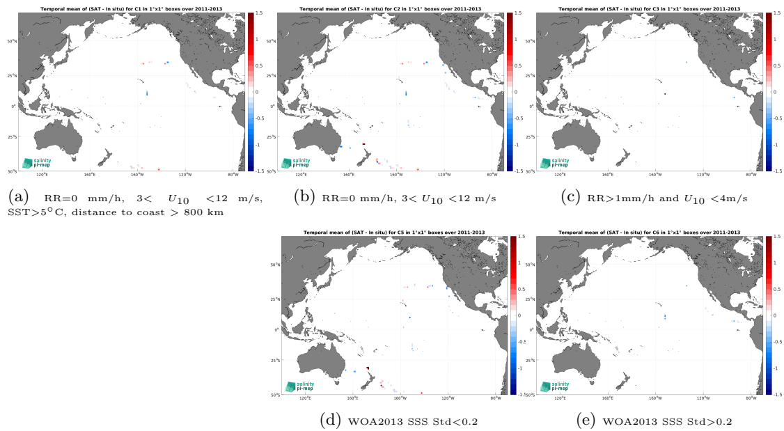
Figure 14: Temporal mean gridded over spatial boxes of size 1^\circ \times 1^\circ of \Delta SSS (Aquarius SSS L2 OR v5 (NASA-GSFC) - TSG (GOSUD-Sailing-ship)) for 5 different subdatasets corresponding to: RR=0 mm/h, 3 < U_{10} < 12 m/s, SST > 5^\circ\text{C} , distance to coast > 800 km (a), RR=0 mm/h, 3 < U_{10} < 12 m/s (b), RR > 1 mm/h and U_{10} < 4 m/s (c), WOA2013 SSS Std < 0.2 (d), WOA2013 SSS Std > 0.2 (e).
