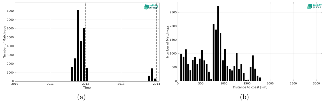
Figure 2: Number of match-ups between TSG (GOSUD-Sailing-ship) and Aquarius SSS L2 OR v5 (NASA-GSFC) SSS as a function of time (a) and as function of the distance to coast (b) over the Pacific Ocean Pi-MEP region and for the full satellite product period.
