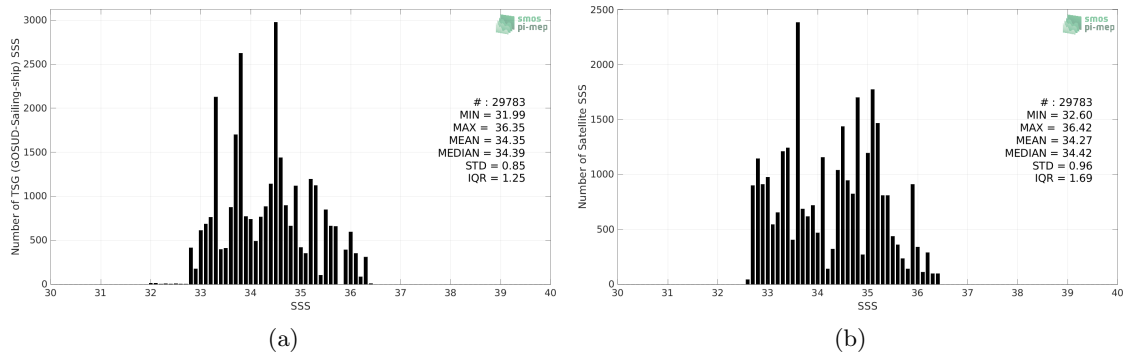
Figure 2: Histograms of SSS from TSG (GOSUD-Sailing-ship) (a) and Aquarius SSS L2 OR v5 (NASA-GSFC) (b) considering all match-up pairs per bins of 0.1 over the Pacific Ocean Pi-MEP region and for the full satellite product period.
