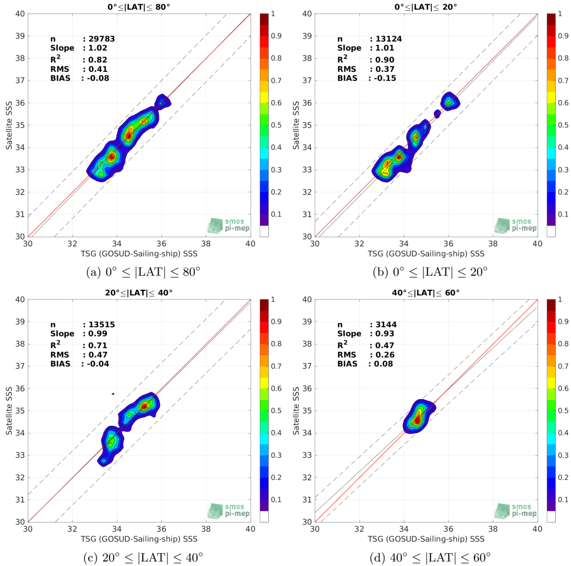
Figure 9: Contour maps of the concentration of Aquarius SSS L2 OR v5 (NASA-GSFC) SSS (y-axis) versus TSG (GOSUD-Sailing-ship) SSS (x-axis) at match-up pairs for different latitude bands. For each plot, the red line shows x=y . The black thin and dashed lines indicate a linear fit through the data cloud and the \pm 95\% confidence levels, respectively. The number match-up pairs n , the slope and R^2 coefficient of the linear fit, the root mean square (RMS) and the mean bias between satellite and in situ data are indicated for each latitude band in each plots.
