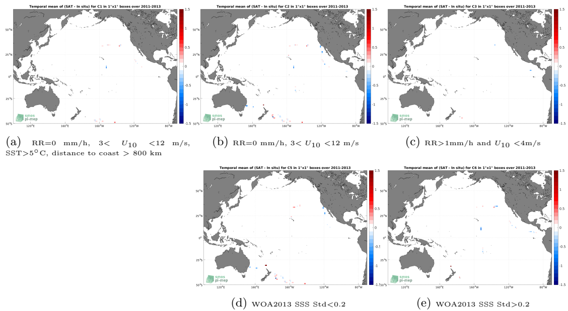
Figure 12: Temporal mean gridded over spatial boxes of size 1^\circ \times 1^\circ of \Delta SSS (Aquarius SSS L2 OR v5 (NASA-GSFC) - TSG (GOSUD-Sailing-ship)) for 5 different subdatasets corresponding to: RR=0 mm/h, 3 < U_{10} < 12 m/s, SST > 5^\circ\text{C} , distance to coast > 800 km (a), RR=0 mm/h, 3 < U_{10} < 12 m/s (b), RR > 1 mm/h and U_{10} < 4 m/s (c), WOA2013 SSS Std < 0.2 (d), WOA2013 SSS Std > 0.2 (e).
