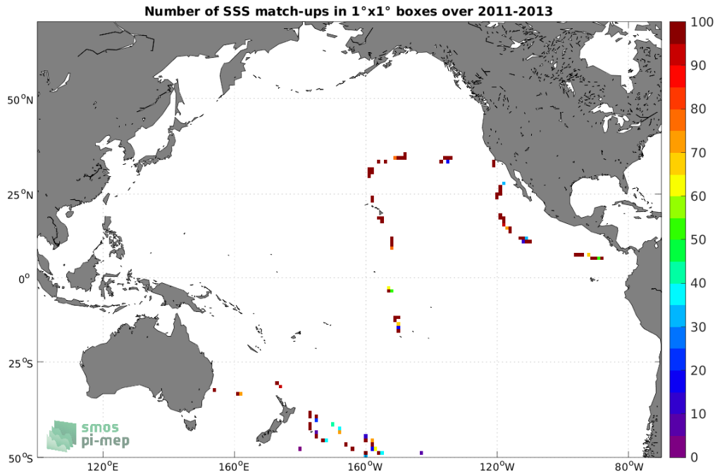
Figure 4: Number of SSS match-ups between TSG (GOSUD-Sailing-ship) SSS and the Aquarius SSS L2 OR v5 (NASA-GSFC) SSS product for the Pacific Ocean Pi-MEP region over 1^\circ \times 1^\circ boxes and for the full satellite product period.
