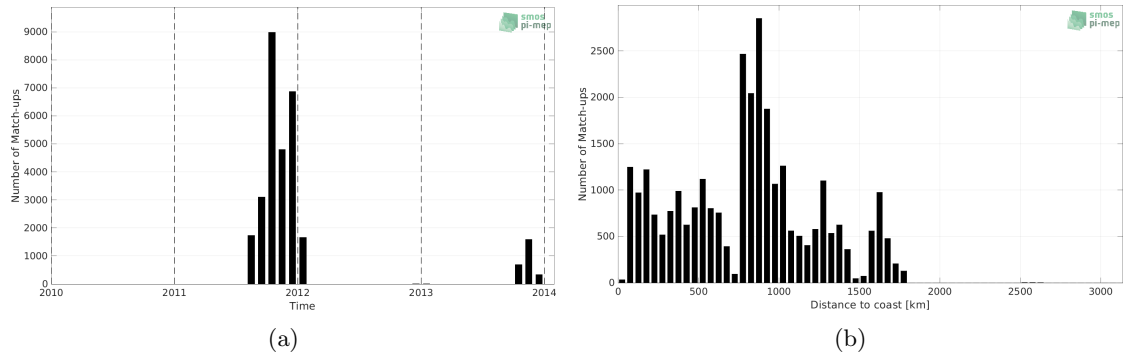
Figure 1: Number of match-ups between TSG (GOSUD-Sailing-ship) and Aquarius SSS L2 OR v5 (NASA-GSFC) SSS as a function of time (a) and as function of the distance to coast (b) over the Pacific Ocean Pi-MEP region and for the full satellite product period.
