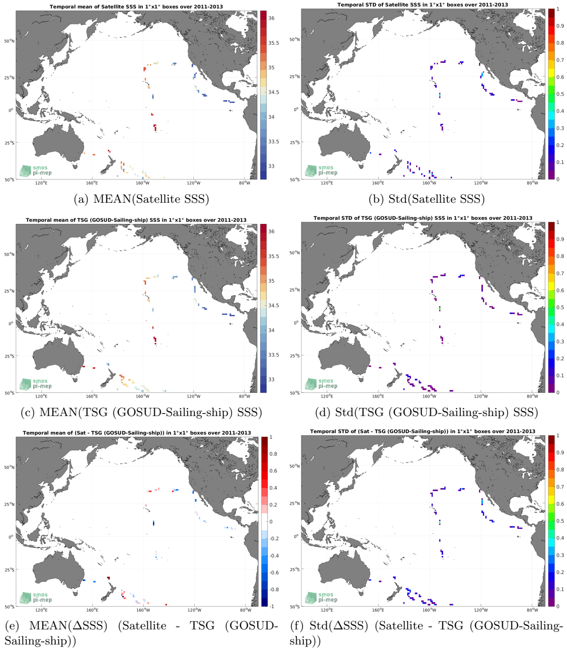
Figure 6: Temporal mean (left) and Std (right) of SSS from Aquarius SSS L2 OR v5 (NASA-GSFC) (top), TSG (GOSUD-Sailing-ship) (middle), and of \Delta SSS (Satellite - TSG (GOSUD-Sailing-ship)). Only match-up pairs are used to generate these maps.
