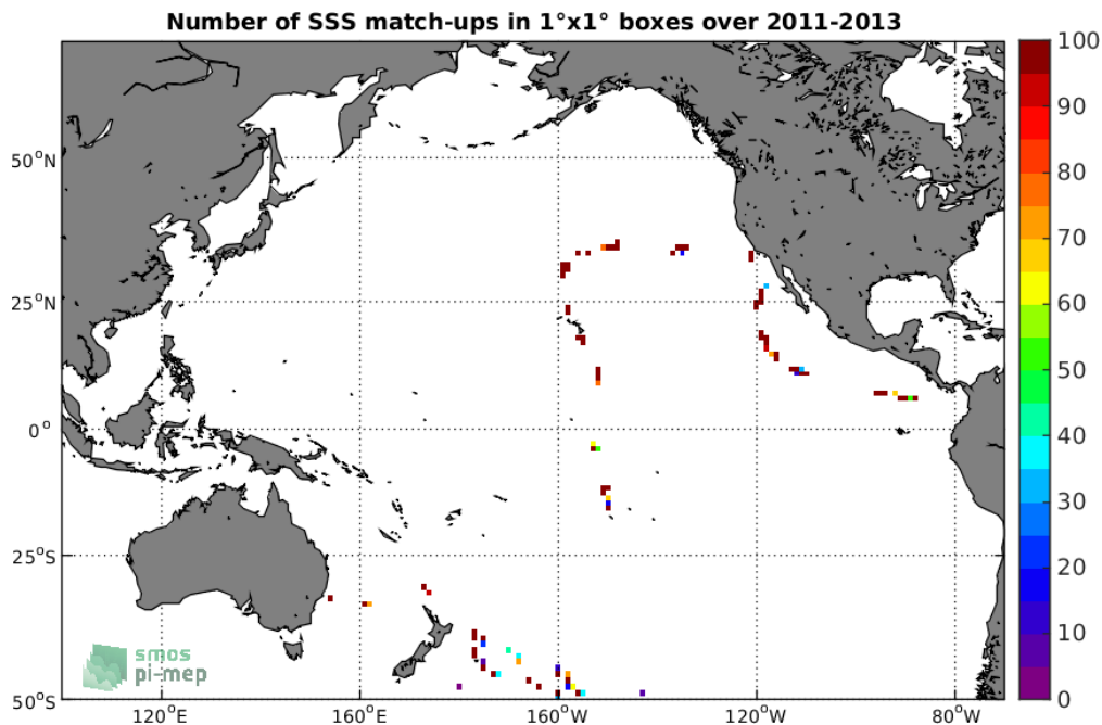
Figure 4: Number of SSS match-ups between TSG-GOSUD-Sailing-ship SSS and the Aquarius-L2-OR-V5 SSS product for the Pacific Ocean Pi-MEP region over 1^\circ \times 1^\circ boxes and for the full satellite product period.
