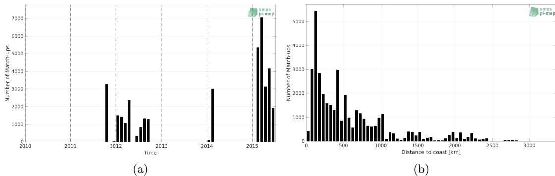
Figure 1: Number of match-ups between TSG (GOSUD-Research-vessel) and Aquarius SSS L2 OR v5 (NASA-GSFC) SSS as a function of time (a) and as function of the distance to coast (b) over the Pacific Ocean Pi-MEP region and for the full satellite product period.
