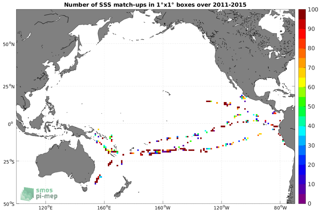
Figure 4: Number of SSS match-ups between TSG (GOSUD-Research-vessel) SSS and the Aquarius SSS L2 OR v5 (NASA-GSFC) SSS product for the Pacific Ocean Pi-MEP region over 1^\circ \times 1^\circ boxes and for the full satellite product period.
