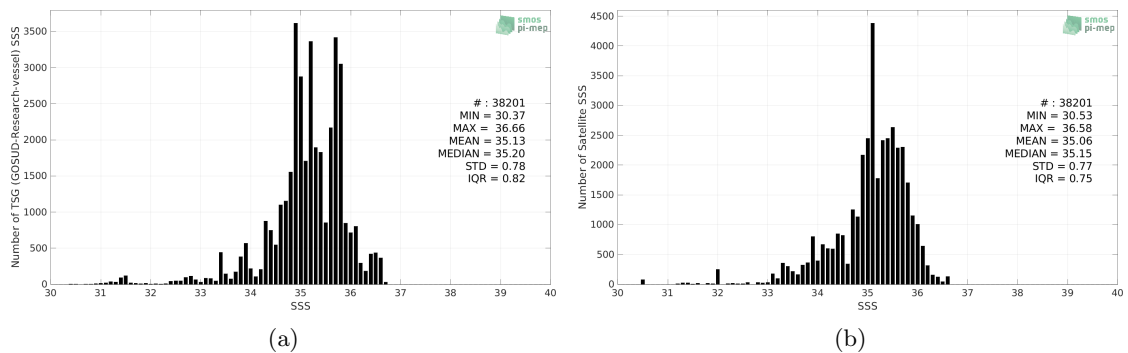
Figure 2: Histograms of SSS from TSG (GOSUD-Research-vessel) (a) and Aquarius SSS L2 OR v5 (NASA-GSFC) (b) considering all match-up pairs per bins of 0.1 over the Pacific Ocean Pi-MEP region and for the full satellite product period.
