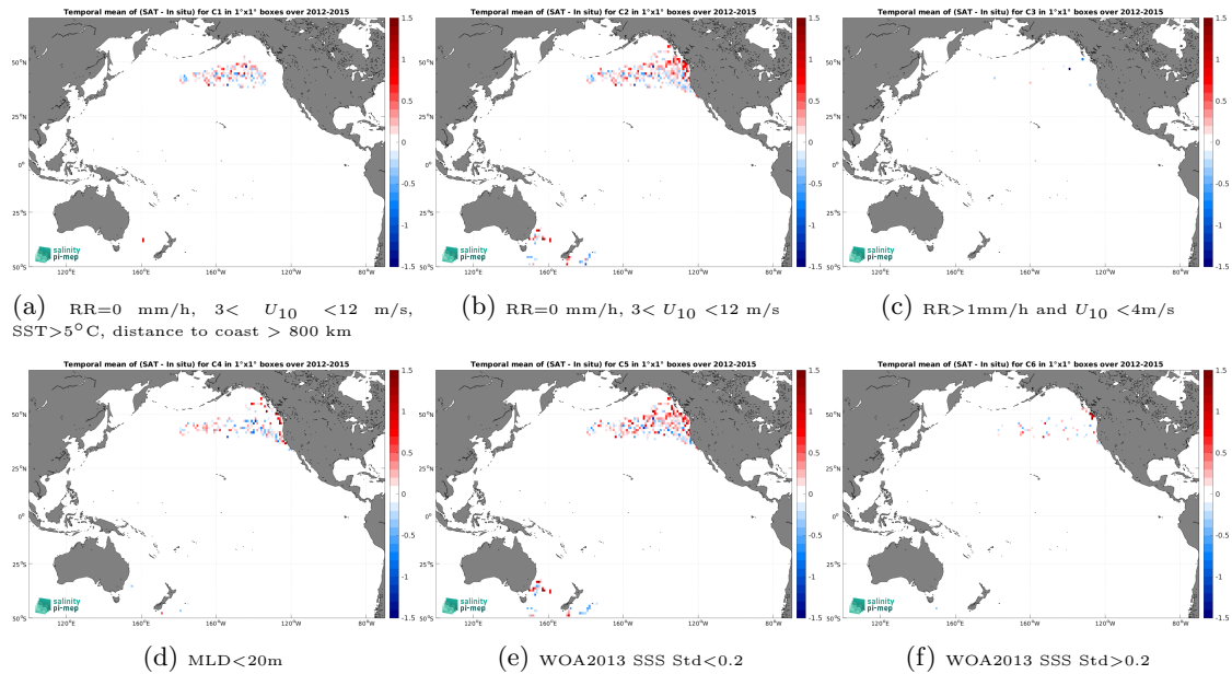
Figure 14: Temporal mean gridded over spatial boxes of size 1^\circ \times 1^\circ of \Delta SSS (Aquarius SSS L2 OR v5 (NASA-GSFC) - Marine mammals) for 6 different subdatasets corresponding to:RR=0 mm/h, 3 < U_{10} < 12 m/s, SST > 5^\circ\text{C} , distance to coast > 800 km (a), RR=0 mm/h, 3 < U_{10} < 12 m/s (b), RR > 1 mm/h and U_{10} < 4 m/s (c),MLD < 20 m (d),WOA2013 SSS Std < 0.2 (e),WOA2013 SSS Std > 0.2 (f).
