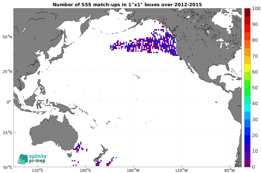
Figure 5: Number of SSS match-ups between Marine mammals SSS and the Aquarius SSS L2 OR v5 (NASA-GSFC) SSS product for the Pacific Ocean Pi-MEP region over 1^\circ \times 1^\circ boxes and for the full satellite product period.
