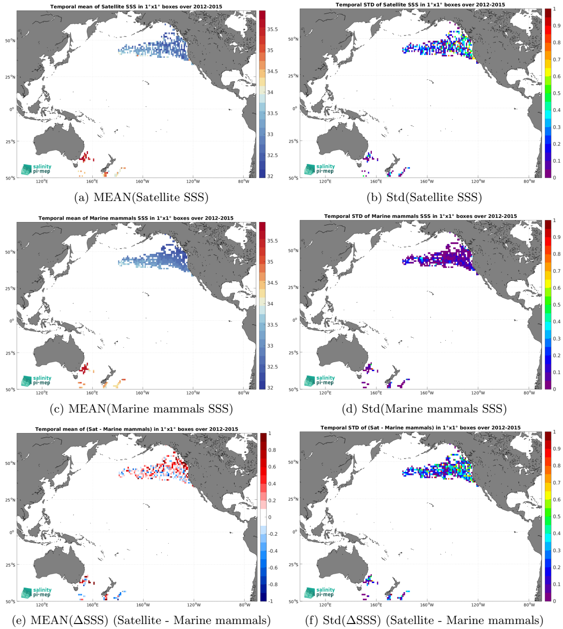
Figure 7: Temporal mean (left) and Std (right) of SSS from Aquarius SSS L2 OR v5 (NASA-GSFC) (top), Marine mammals (middle), and of \Delta SSS (Satellite - Marine mammals). Only match-up pairs are used to generate these maps.
