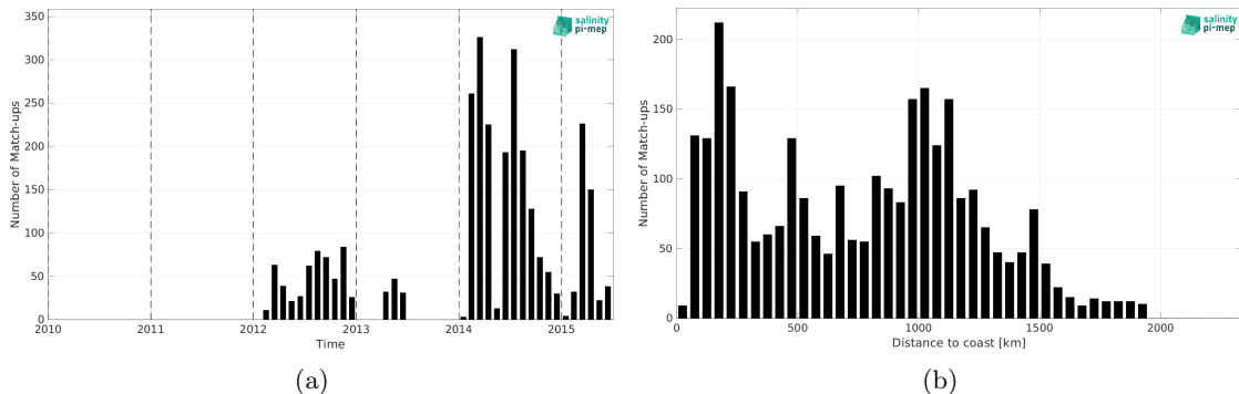
Figure 2: Number of match-ups between Marine mammals and Aquarius SSS L2 OR v5 (NASA-GSFC) SSS as a function of time (a) and as function of the distance to coast (b) over the Pacific Ocean Pi-MEP region and for the full satellite product period.
