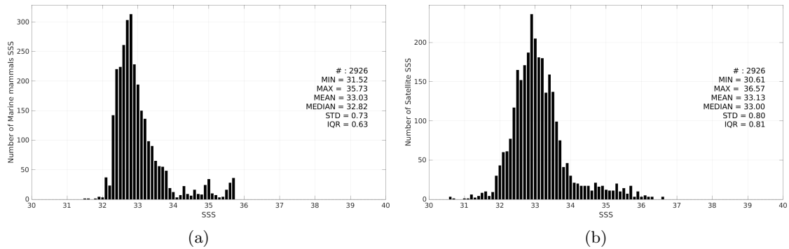
Figure 3: Histograms of SSS from Marine mammals (a) and Aquarius SSS L2 OR v5 (NASA-GSFC) (b) considering all match-up pairs per bins of 0.1 over the Pacific Ocean Pi-MEP region and for the full satellite product period.
