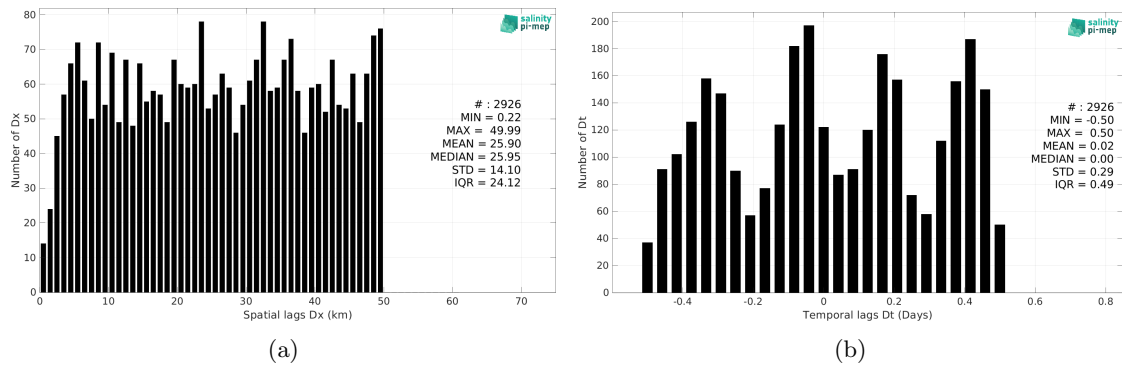
Figure 6: Histograms of the spatial (a) and temporal (b) lags between the location/time of the Marine mammals measurement and the date of the corresponding Aquarius SSS L2 OR v5 (NASA-GSFC) SSS pixel.
