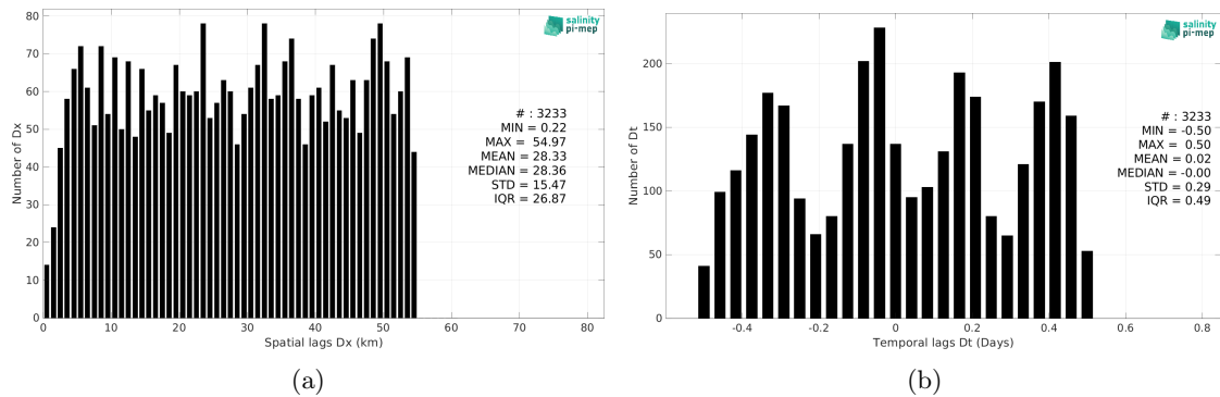
Figure 5: Histograms of the spatial (a) and temporal (b) lags between the location/time of the Marine mammals measurement and the date of the corresponding Aquarius SSS L2 OR v5 (NASA-GSFC) SSS pixel.
