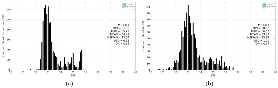
Figure 2: Histograms of SSS from Marine mammals (a) and Aquarius SSS L2 OR v5 (NASA-GSFC) (b) considering all match-up pairs per bins of 0.1 over the Pacific Ocean Pi-MEP region and for the full satellite product period.
