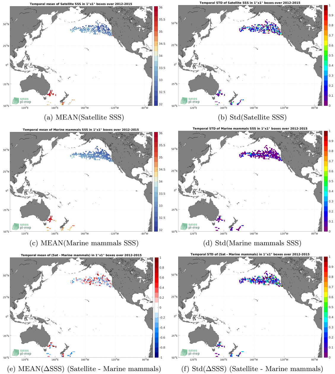
Figure 6: Temporal mean (left) and Std (right) of SSS from Aquarius SSS L2 OR v5 (NASA-GSFC) (top), Marine mammals (middle), and of \Delta SSS (Satellite - Marine mammals). Only match-up pairs are used to generate these maps.
