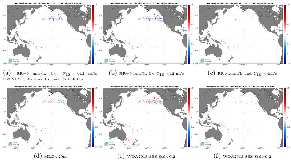
Figure 12: Temporal mean gridded over spatial boxes of size 1^\circ \times 1^\circ of \Delta SSS (Aquarius SSS L2 OR v5 (NASA-GSFC) - Marine mammals) for 6 different subdatasets corresponding to:RR=0 mm/h, 3 < U_{10} < 12 m/s, SST > 5^\circ\text{C} , distance to coast > 800 km (a), RR=0 mm/h, 3 < U_{10} < 12 m/s (b), RR > 1 mm/h and U_{10} < 4 m/s (c),MLD < 20 m (d),WOA2013 SSS Std < 0.2 (e),WOA2013 SSS Std > 0.2 (f).
