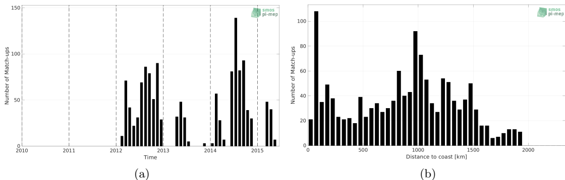
Figure 1: Number of match-ups between Marine mammals and Aquarius SSS L2 OR v5 (NASA-GSFC) SSS as a function of time (a) and as function of the distance to coast (b) over the Pacific Ocean Pi-MEP region and for the full satellite product period.
