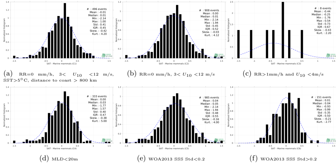
Figure 13: Normalized histogram of \Delta\text{SSS} (Aquarius SSS L2 OR v5 (NASA-GSFC) - Marine mammals) for 6 different subdatasets corresponding to: RR=0 mm/h, 3 < U_{10} < 12 m/s, SST>5°C, distance to coast > 800 km (a), RR=0 mm/h, 3 < U_{10} < 12 m/s (b), RR>1mm/h and U_{10} < 4 m/s (c), MLD<20m (d), WOA2013 SSS Std<0.2 (e), WOA2013 SSS Std>0.2 (f).
