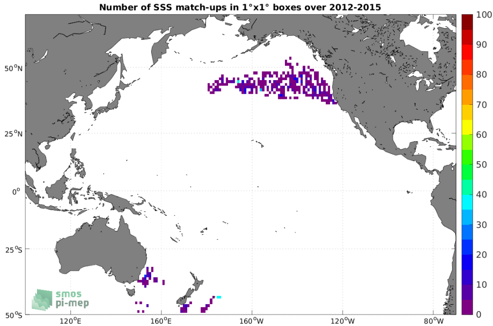
Figure 4: Number of SSS match-ups between Marine mammals SSS and the Aquarius SSS L2 OR v5 (NASA-GSFC) SSS product for the Pacific Ocean Pi-MEP region over 1^\circ \times 1^\circ boxes and for the full satellite product period.
