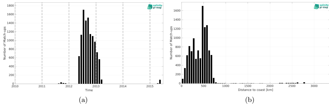
Figure 2: Number of match-ups between Surface drifters and Aquarius SSS L2 OR v5 (NASA-GSFC) SSS as a function of time (a) and as function of the distance to coast (b) over the Pacific Ocean Pi-MEP region and for the full satellite product period.
