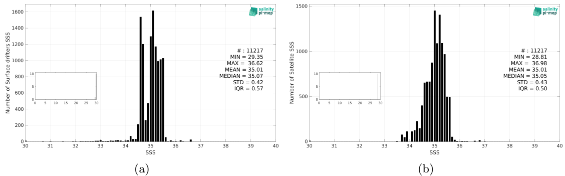
Figure 3: Histograms of SSS from Surface drifters (a) and Aquarius SSS L2 OR v5 (NASA-GSFC) (b) considering all match-up pairs per bins of 0.1 over the Pacific Ocean Pi-MEP region and for the full satellite product period.
