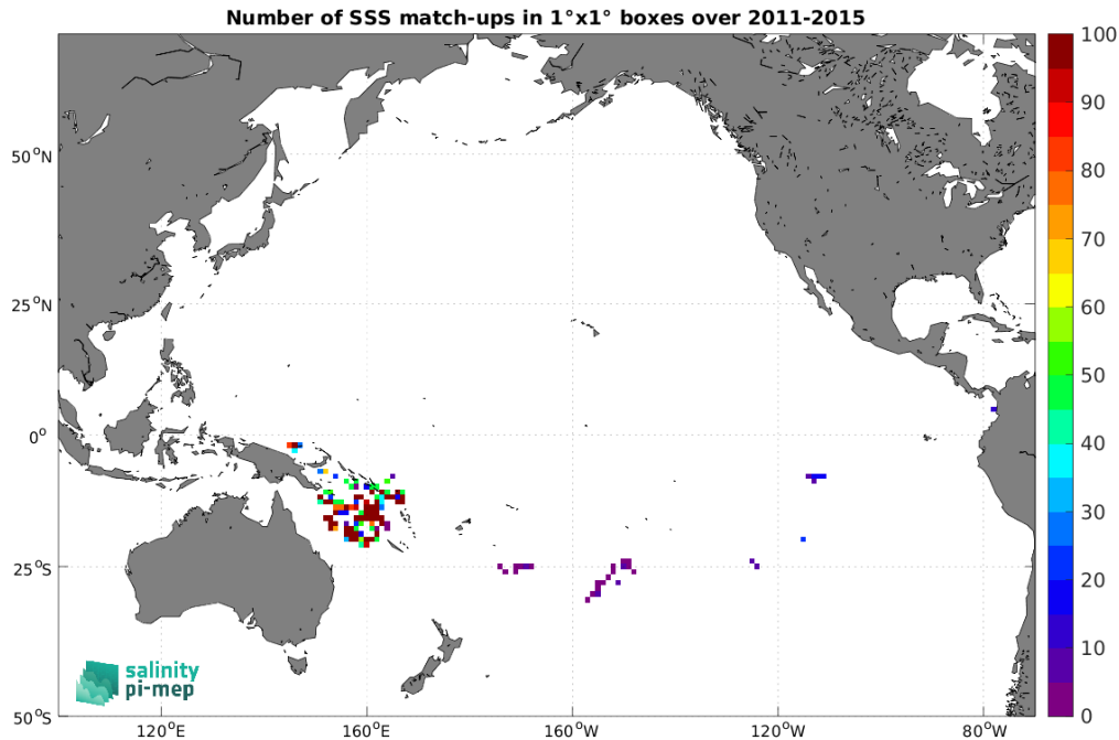
Figure 4: Number of SSS match-ups between Surface drifters SSS and the Aquarius SSS L2 OR v5 (NASA-GSFC) SSS product for the Pacific Ocean Pi-MEP region over 1^\circ \times 1^\circ boxes and for the full satellite product period.
