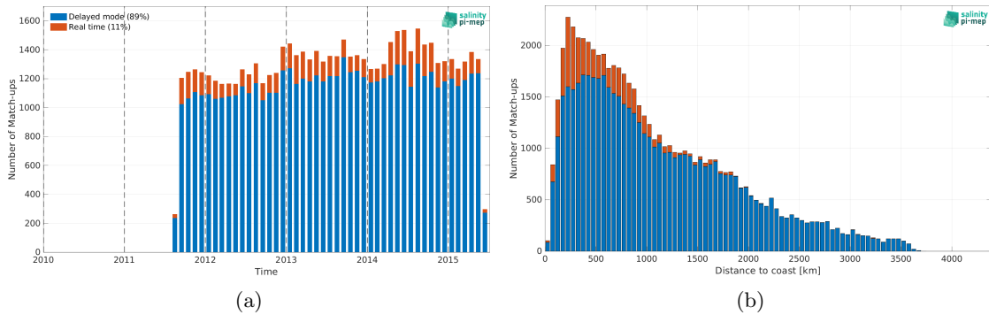
Figure 2: Number of match-ups between Argo and Aquarius SSS L2 OR v5 (NASA-GSFC) SSS as a function of time (a) and as function of the distance to coast (b) over the Pacific Ocean Pi-MEP region and for the full satellite product period.
