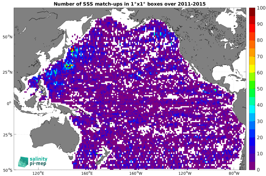
Figure 5: Number of SSS match-ups between Argo SSS and the Aquarius SSS L2 OR v5 (NASA-GSFC) SSS product for the Pacific Ocean Pi-MEP region over 1^\circ \times 1^\circ boxes and for the full satellite product period.
