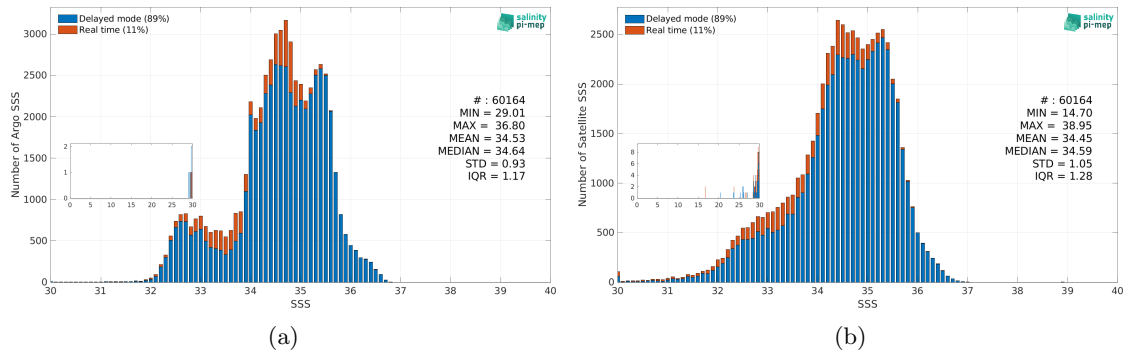
Figure 3: Histograms of SSS from Argo (a) and Aquarius SSS L2 OR v5 (NASA-GSFC) (b) considering all match-up pairs per bins of 0.1 over the Pacific Ocean Pi-MEP region and for the full satellite product period.
