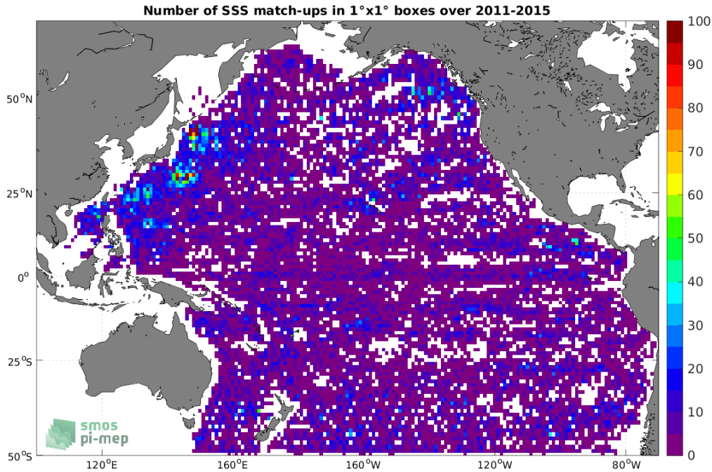
Figure 4: Number of SSS match-ups between Argo SSS and the Aquarius SSS L2 OR v5 (NASA-GSFC) SSS product for the Pacific Ocean Pi-MEP region over 1°x1° boxes and for the full satellite product period.
