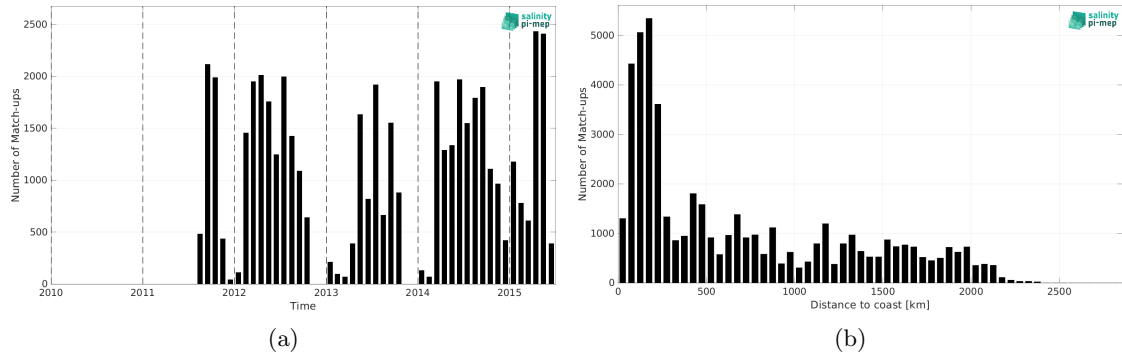
Figure 2: Number of match-ups between TSG (SAMOS) and Aquarius SSS L2 CAP v5 (JPL) SSS as a function of time (a) and as function of the distance to coast (b) over the Pacific Ocean Pi-MEP region and for the full satellite product period.
