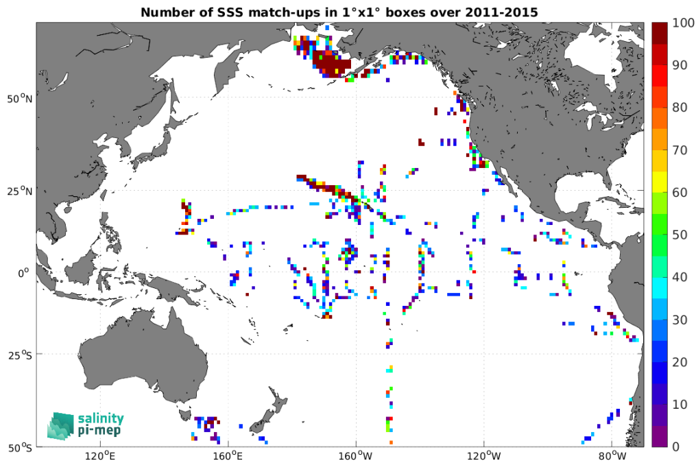
Figure 5: Number of SSS match-ups between TSG (SAMOS) SSS and the Aquarius SSS L2 CAP v5 (JPL) SSS product for the Pacific Ocean Pi-MEP region over 1^\circ \times 1^\circ boxes and for the full satellite product period.
