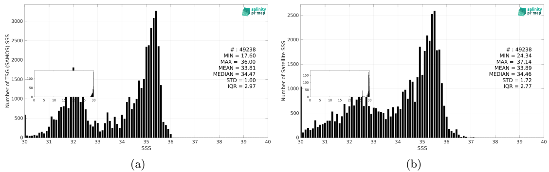
Figure 3: Histograms of SSS from TSG (SAMOS) (a) and Aquarius SSS L2 CAP v5 (JPL) (b) considering all match-up pairs per bins of 0.1 over the Pacific Ocean Pi-MEP region and for the full satellite product period.
