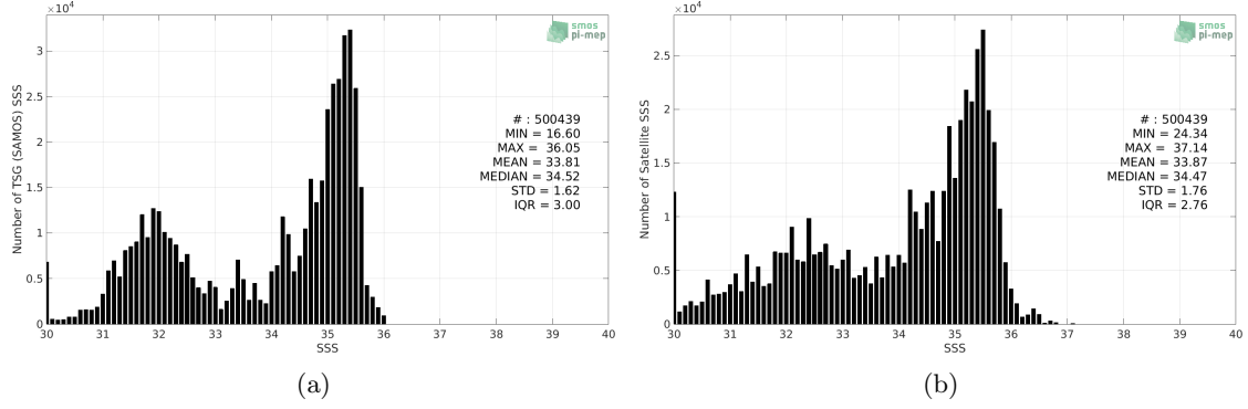
Figure 2: Histograms of SSS from TSG (SAMOS) (a) and Aquarius SSS L2 CAP v5 (JPL) (b) considering all match-up pairs per bins of 0.1 over the Pacific Ocean Pi-MEP region and for the full satellite product period.
