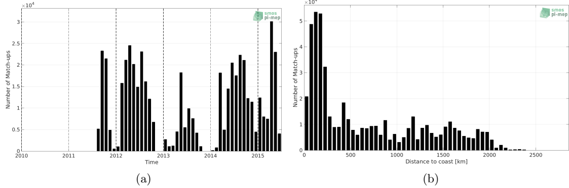
Figure 1: Number of match-ups between TSG (SAMOS) and Aquarius SSS L2 CAP v5 (JPL) SSS as a function of time (a) and as function of the distance to coast (b) over the Pacific Ocean Pi-MEP region and for the full satellite product period.
