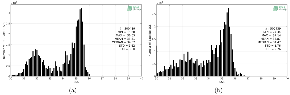
Figure 2: Histograms of SSS from TSG-SAMOS (a) and Aquarius-L2-JPL-V5 (b) considering all match-up pairs per bins of 0.1 over the Pacific Ocean Pi-MEP region and for the full satellite product period.
